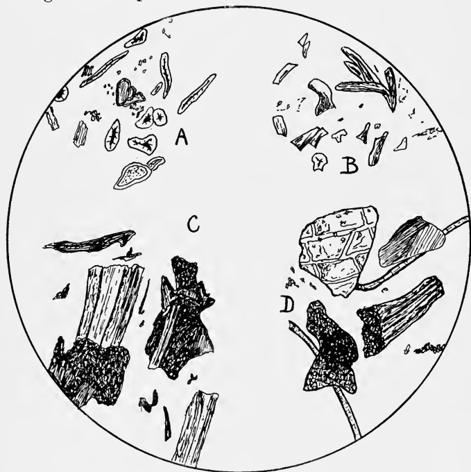
FIG. 10.—Micrograph showing appearance of (A) Ground Coconut Shell, (B) Ground Olive Stones, (C) Wood Dust and (D) Cocoa Shell Powder.
