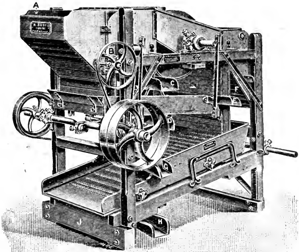
Boby's patent linseed dresser (belt driven). Cleans up to 80 bushels of linseed per hour, separating weed seeds, rubbish and dust.
