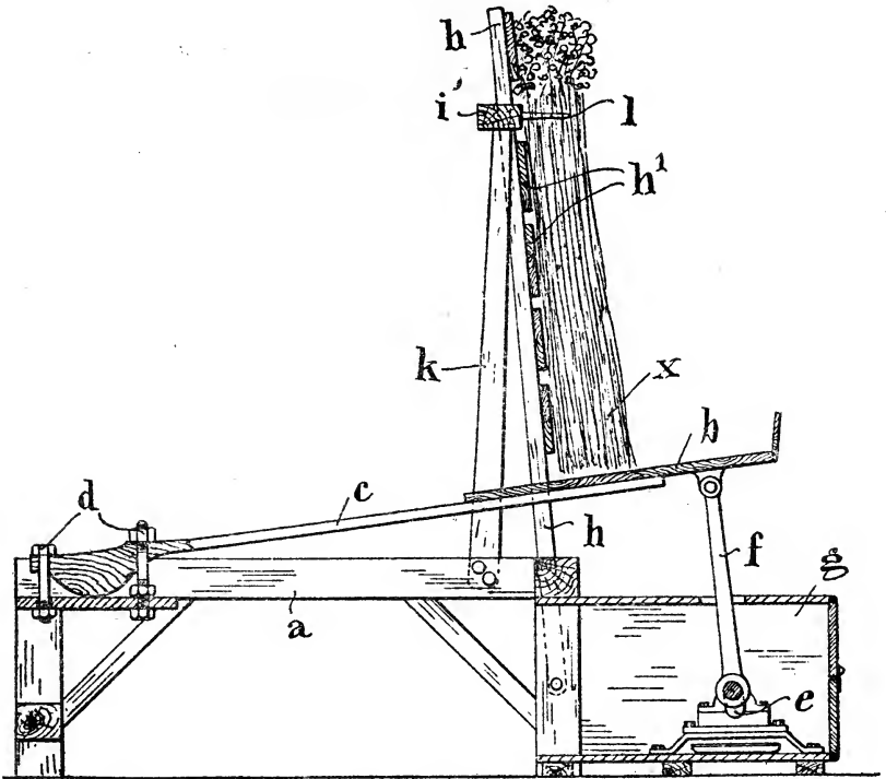
Butting or root levelling machine for flax straw.
