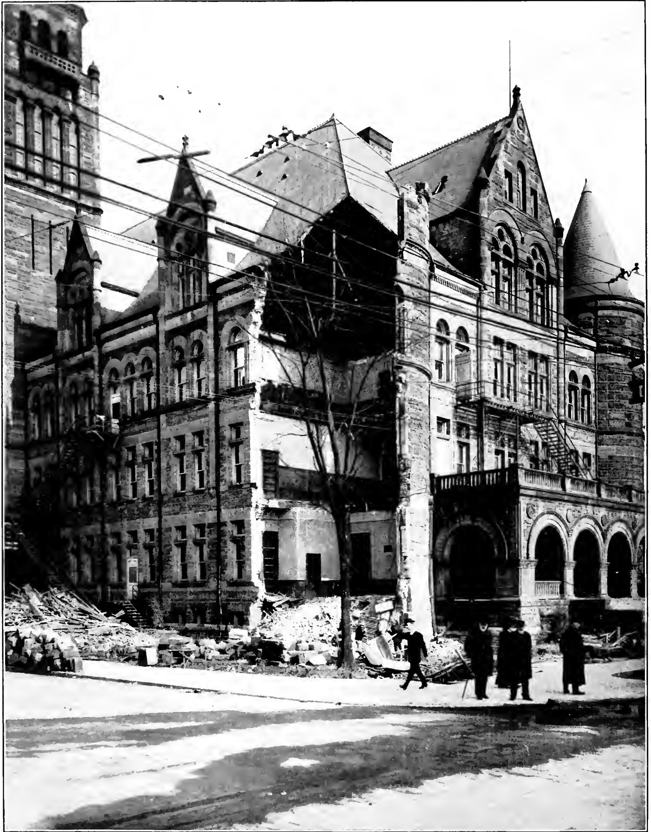
FIG. 10.—STEELE HIGH SCHOOL BUILDING, DAYTON, OHIO. Showing destruction due to undermining foundation by water.
