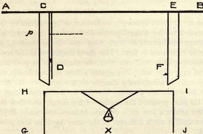
FIG. 25. ARRANGEMENT FOR MEASURING STRENGTH OF FILM.
