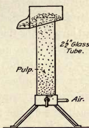
FIG. 74. QUALITATIVE OIL TESTER.
