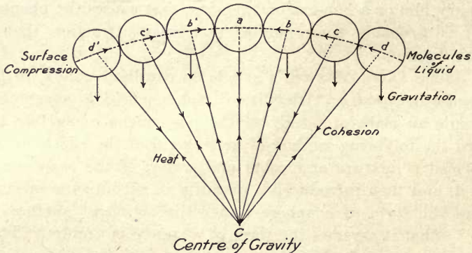
FIG. 76. FORCES AFFECTING SURFACE OF WATER.
