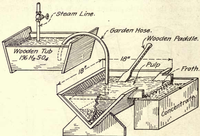
FIG. 57. A POTTER-DELPRAT TEST.
