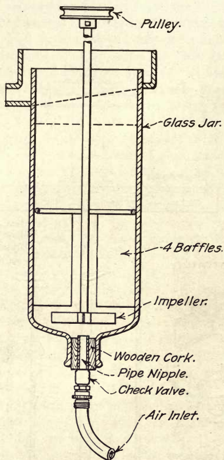
FIG. 69. OWEN TEST-MACHINE.
