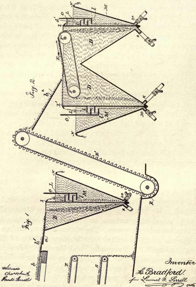
FIG. 2. THE BRADFORD PATENT.
