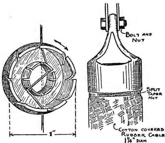
At Left, Substitute for Turnbuckle. At Right, Blieriot's Shock Absorber.
