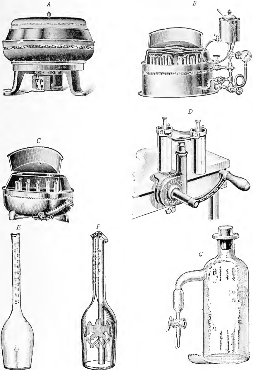
FIG. 45.—Apparatus for Babcock Test.
