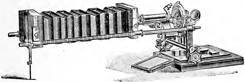
FIG 37b.—Photomicrographic Camera in Horizontal Position
