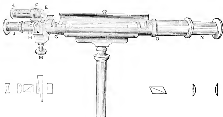
FIG. 102.—Single-wedge Saccharimeter.
