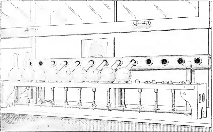
FIG. 270. Johnson Digestion Stand for Nitrogen Determination with Lead Pipe for Carrying off Fumes.
