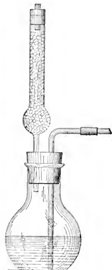
FIG. 69.—Apparatus for Determining Leavening Power of Yeast.
