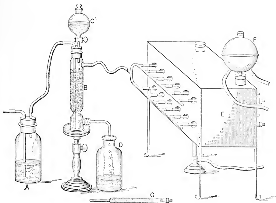
FIG. 18.—Apparatus for Drying in Hydrogen.
