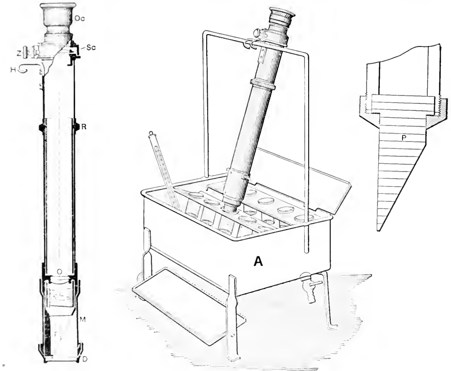
FIG. 42.—The Zeiss Immersion Refractometer.
