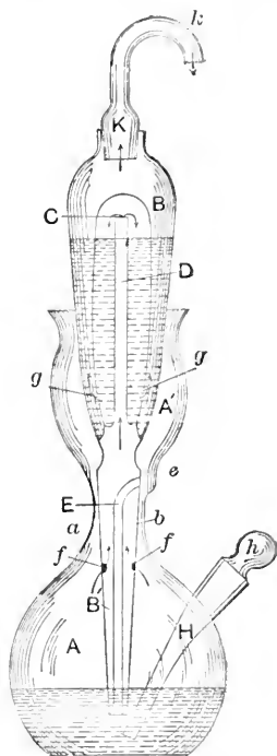
FIG. 78.—Geissler's \text{CO}_2 Apparatus or Alkalimeter.
