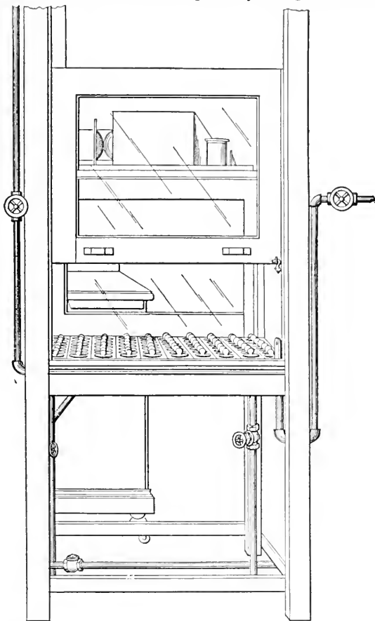
FIG. 7.—Water-bath, Enclosed in Hood, with Sliding-sash Front.
