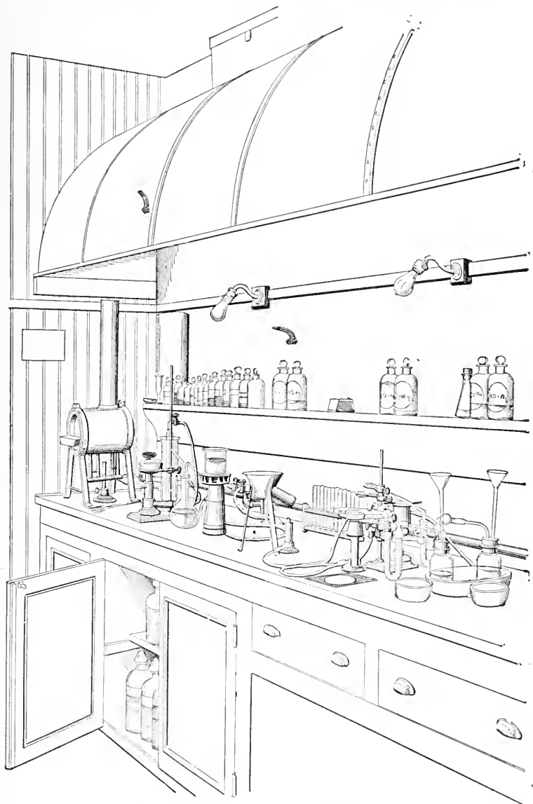
FIG. 3.—Hooded Top of Galvanized Iron over Working-bench, Connected with Ventilating Air-ducts.
