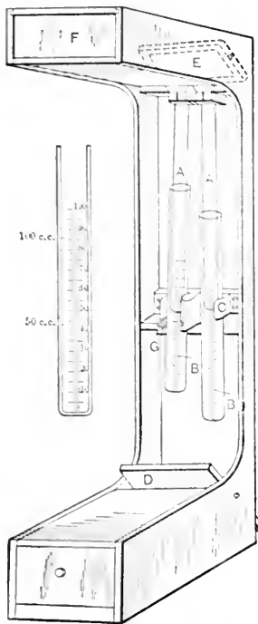
FIG. 30.—Schreiner's Colorimeter with a Tube showing Graduation.
