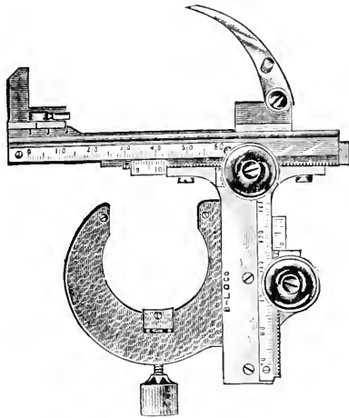
FIG. 33.—Mechanical Stage for Microscope.
