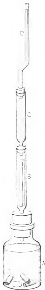
FIG. 29.—Bishop Apparatus for Arsenic.
