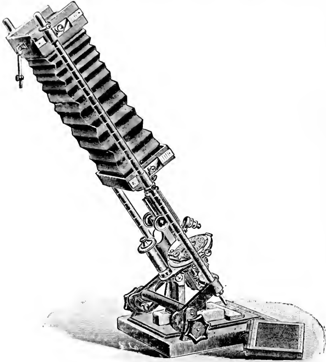
FIG 37a.—A Convenient Photomicrographic Camera.
