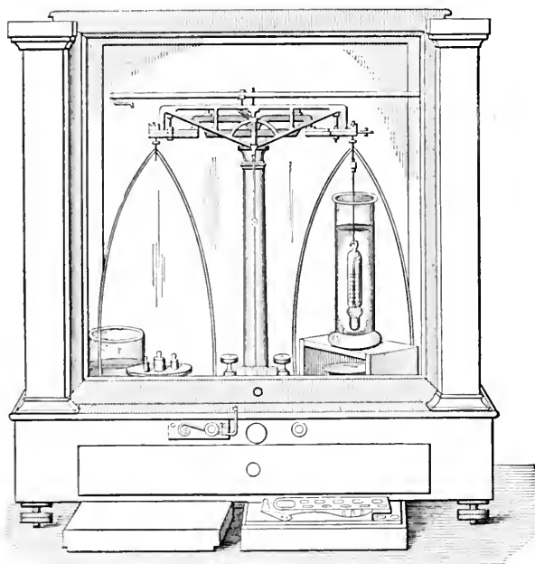
FIG. 15.—The Analytical Balance Arranged for Determining Specific Gravity with the Westphal Plummeter.
