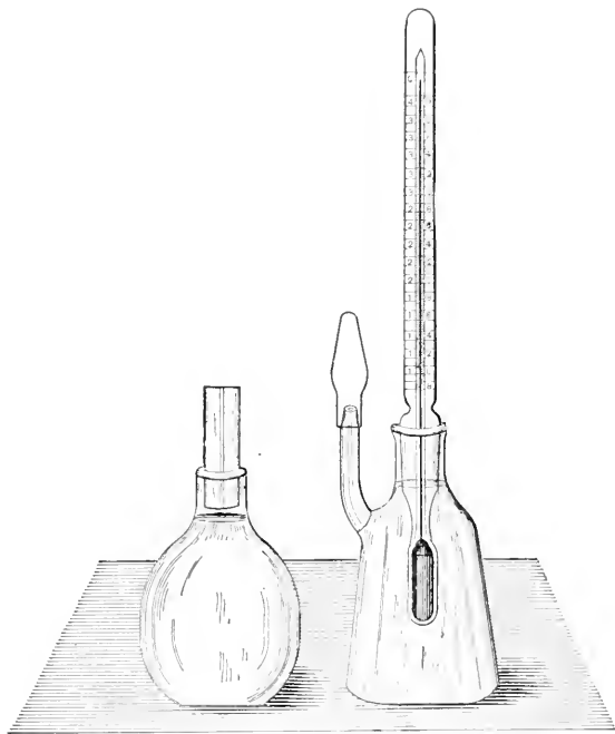
FIG. 16.—Types of Pycnometer.
