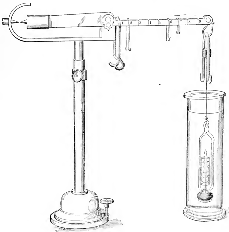
FIG. 14.—The Westphal Balance.
