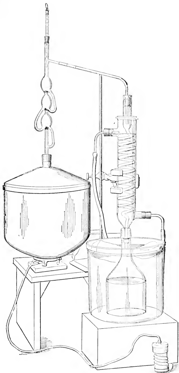
FIG. 23.—Fractionating-still, Arranged for Petroleum Ether.
