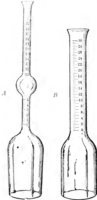
FIG. 5A—Varieties of Babcock Test Bottle for Cream.
