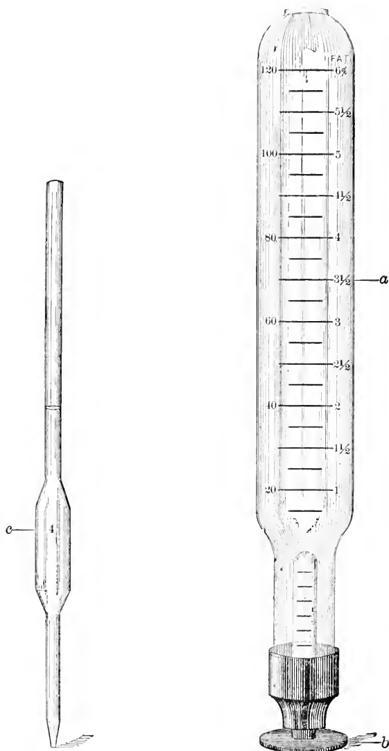
FIG. 50.—Feser's Lactoscope.
