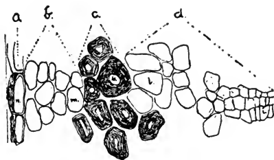
Cross-section of bark of flax plant: a epidermis, b parenchyma, c bast, d cambium. Enlarged 260 times (After Luggier)
