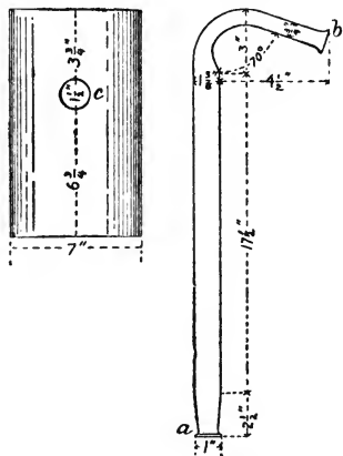
Vertical air blast separator
