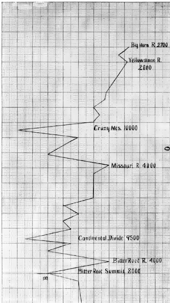
Fig. 4. Section of Idaho-Montana topography along the 46th parallel. B, boundary line. Scale: horizontal, \frac{1}{2} inch = 25 miles; vertical, \frac{1}{2} inch = 1000 feet. O, mean sea level. After topographic maps of the U. S. Geol. Surv.
