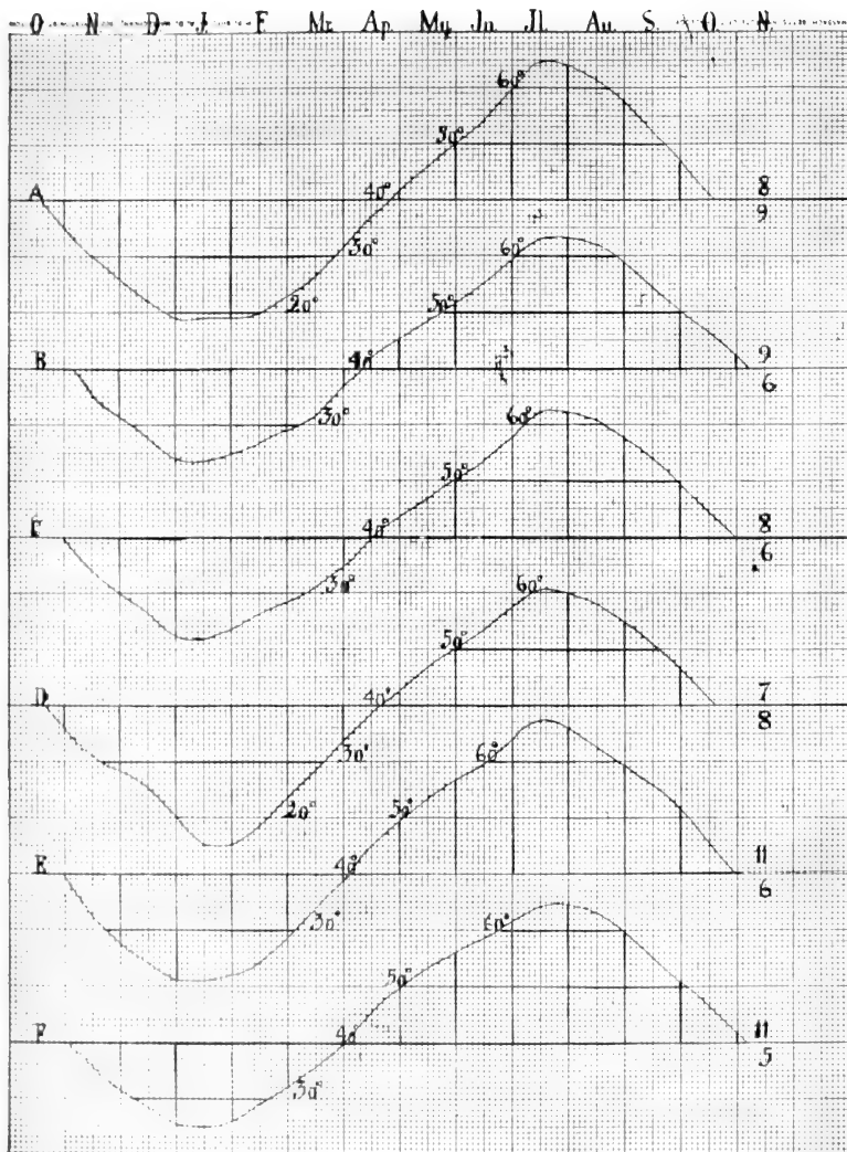
Fig. 8. Mean temperature diagrams for the year. A, Mammoth Hot Springs, Yellowstone Park, altitude 6200 feet. B, Anaconda, altitude, 5300 feet. C, Philipsburg, altitude, 5275 feet. D, Ovando, altitude, 4101 feet. E, Missoula, altitude, 3212 feet. F, Troy, altitude, 1880 feet. The figures at the right represent the ratios of the growing to non-growing seasons. The mean temperatures for the months are on the curves midway between the vertical lines.
