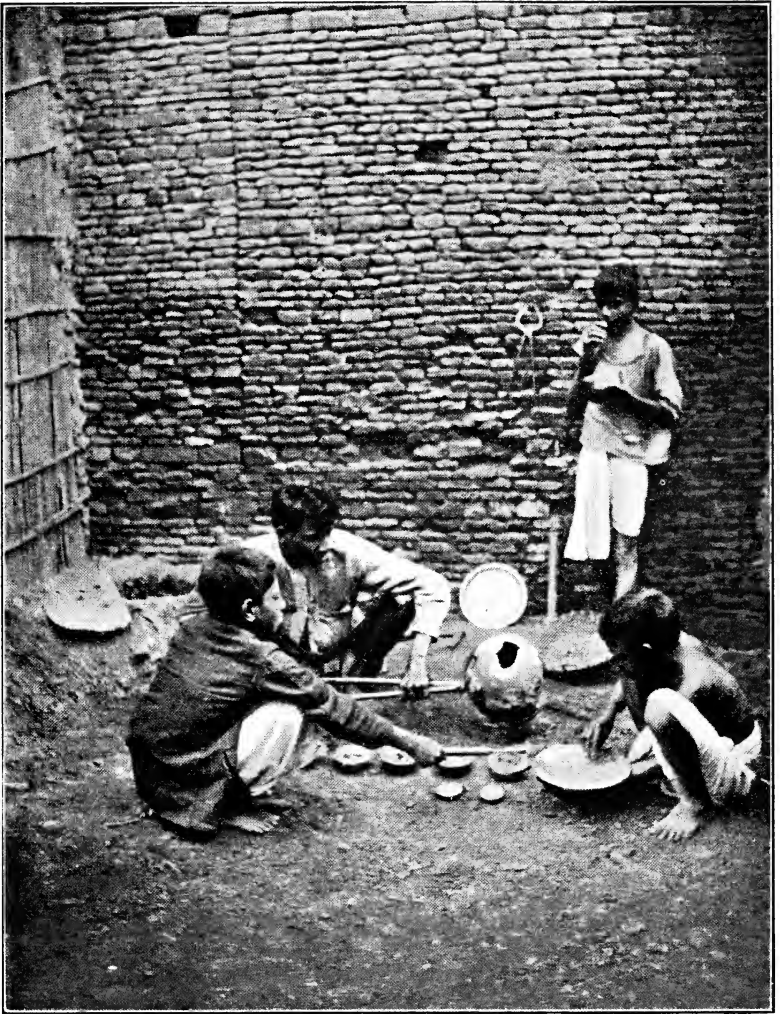
THE FURNACE : THE ARTISAN POURING THE MOLTEN KANSA INTO THE EARTHEN CRUCIBLES.
