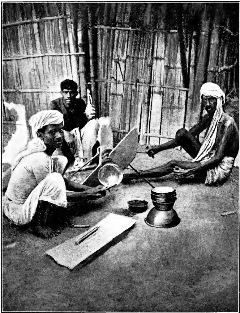
THE HAND-LATHE FOR CHISELLING AND POLISHING: THE ARTISAN APPLYING THE CHISEL TO THE REVOLVING VESSEL.
