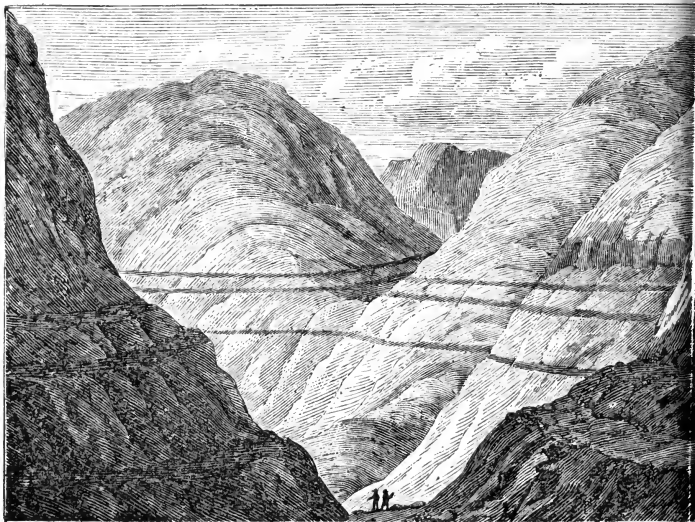
PARALLEL ROADS OF GLEN ROY.
