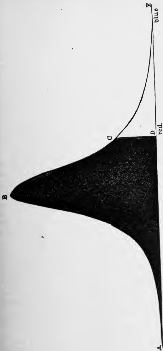
SPECTRUM OF ELECTRIC LIGHT.
