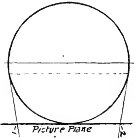
FIG. 60 Perspective of the circles.
