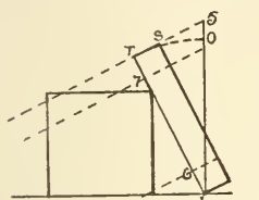
END VIEW OF GROUP. THE LINES WHICH IN FIG. 257 VANISH IN OVP2 ARE HERE SEEN TO BE ACTUALLY PARALLEL.
