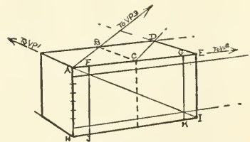
PERSPECTIVE VIEW. THE LINES AB AND CD ARE ACTUALLY PARALLEL AND VANISH IN VP_3 .
