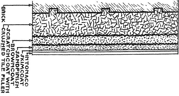
FRESCO GROUNDS CRUSHED TILE FILLER THROWN ON BRICK
