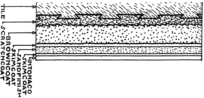
LIME-SAND ON HOLLOW TILE
