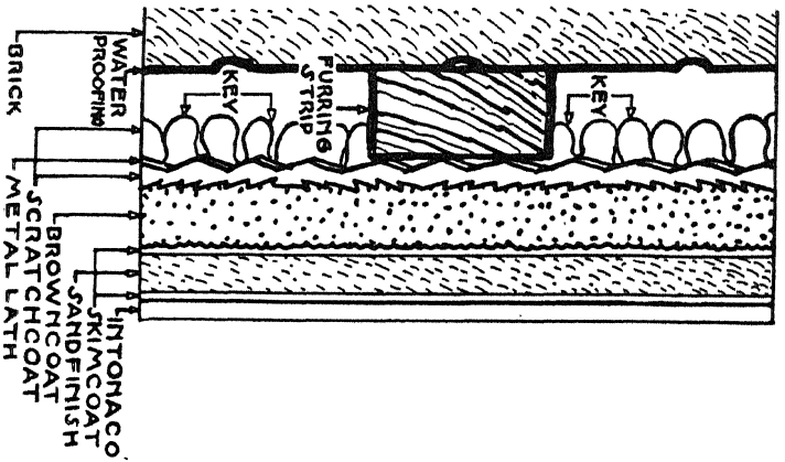
FURRED OUT METAL LATH ON BRICK WALL
