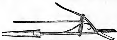
FIG. 154. Grape Gatherer. —
