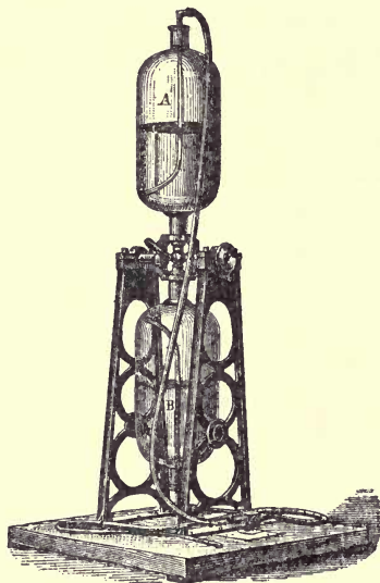
FIG. 14.—MUENCKE'S ASPIRATOR.
