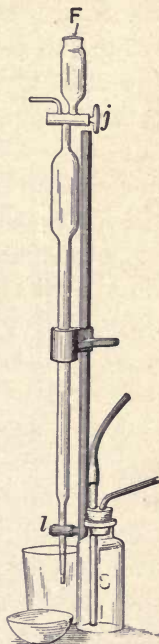
FIG. 9.—BUNTE'S GAS APPARATUS.
