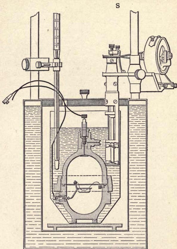
EMERSON-FUEL-CALORIMETER
