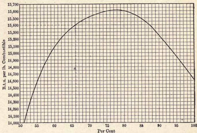
FIG. 18.—CHART FOR DETERMINING HEAT VALUE OF COMBUSTIBLE WITH DIFFERENT PERCENTAGES OF FIXED CARBON.
