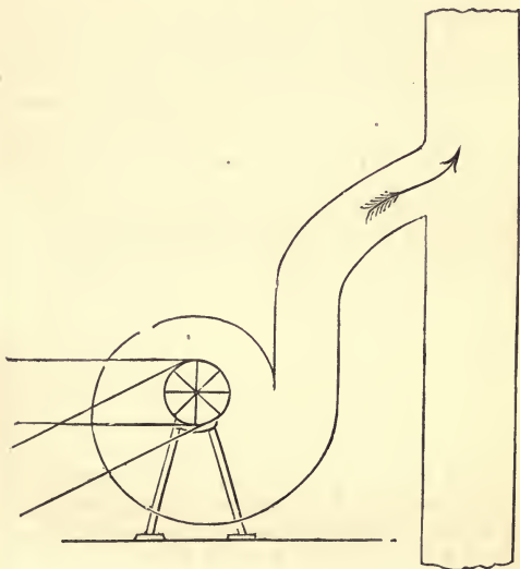
Fig. 97.—Mechanical Draught.
