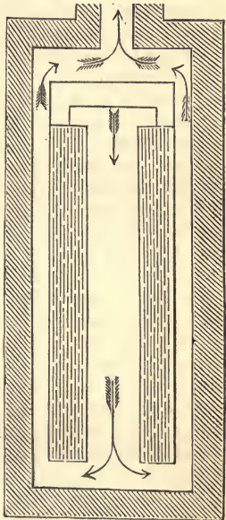
Fig. 96.—Split Draught.
