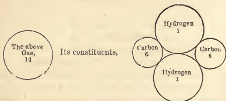
Fig. 2.—Bi-Carburetted Hydrogen.
