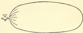
Fig. 104 —Air at 32^{\circ} = 36 grains = 28 nitrogen, 8 oxygen.
