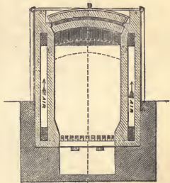
SECTION ON LINE C.D.
