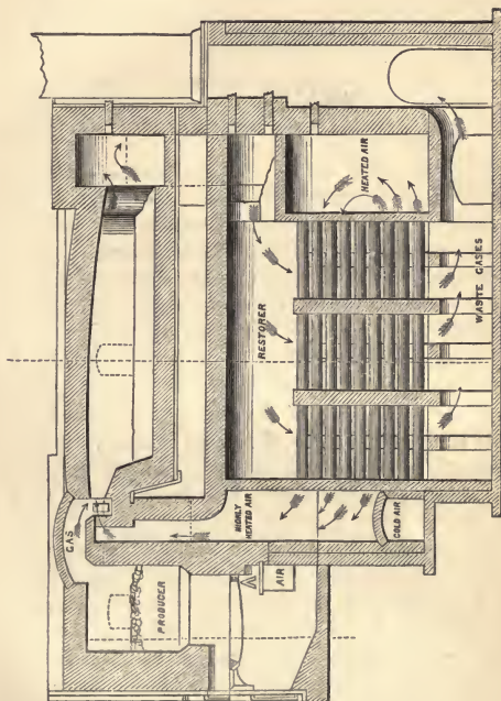
Fig. 139.—Gorman's Heat-restoring Gas-furnace.
