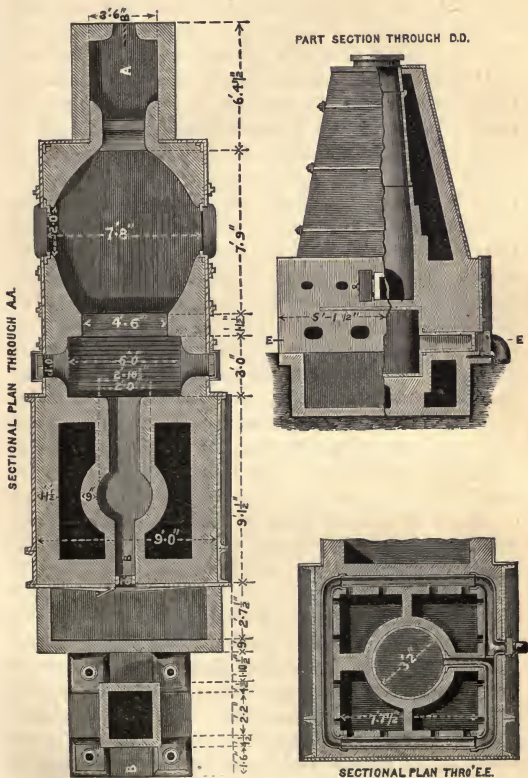
Figs. 130.—Price's Retort Furnace.
