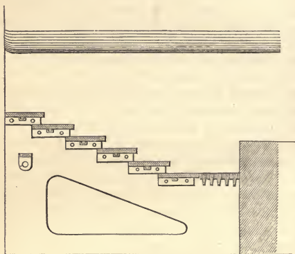
Fig. 117.—Step-Grate.
