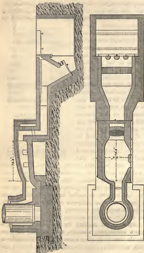
Figs. 127.—The Bicheroux Puddling Furnace.
