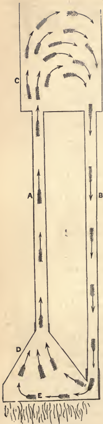
Fig. 72.—Ebullition.
