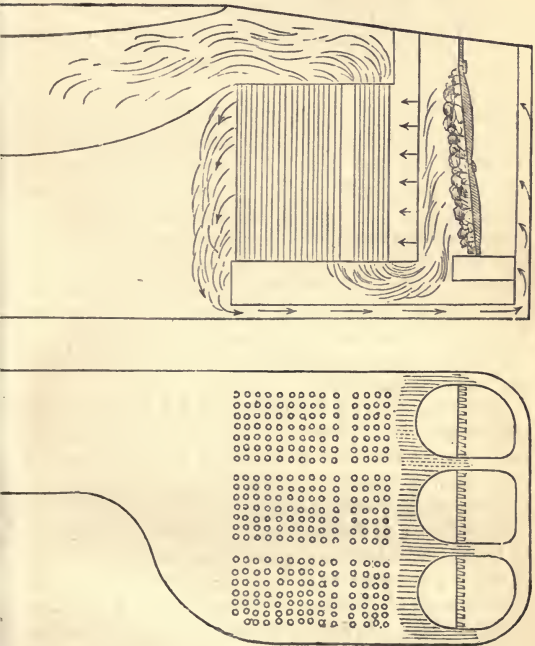
Fig. 100.—Marine Boiler.
