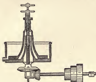
FIG. 7. CLEAN-UP PAN.
