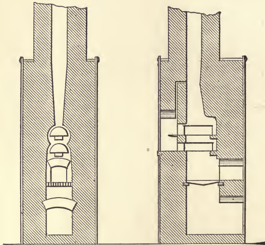
MUFFLE FURNACE FOR BITUMINOUS COAL Scale \frac{1}{4} in. = 1 ft.
