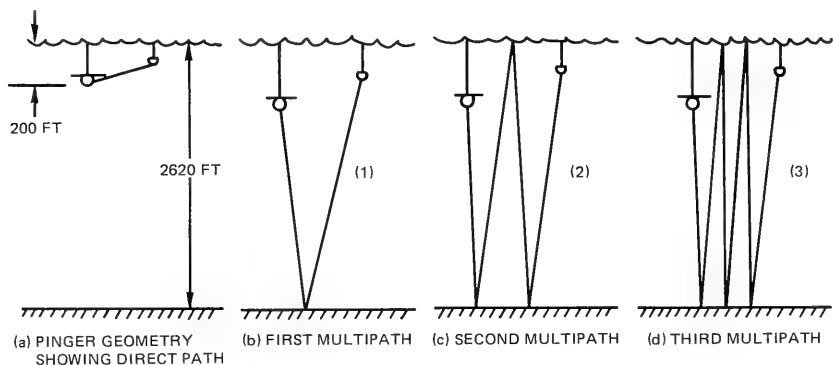
Figure 10. 9-kHz pinger geometry.
