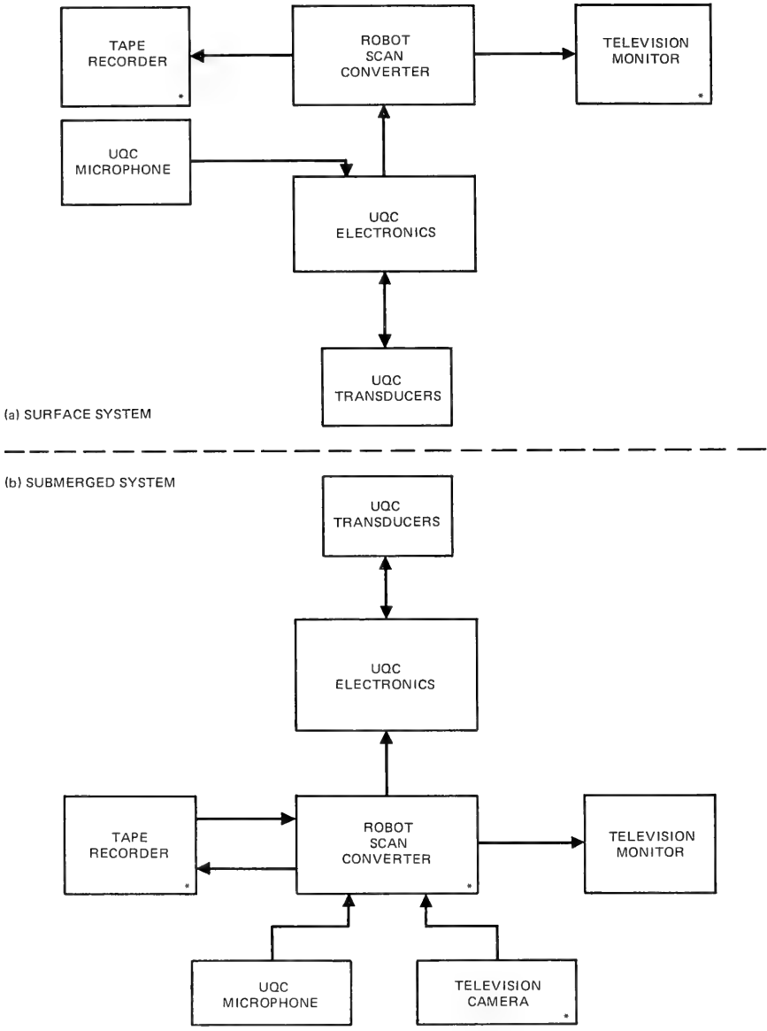
Figure 2. System interconnection diagram.
