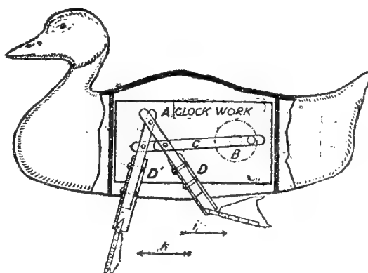
Mechanism that makes the duck paddle.
