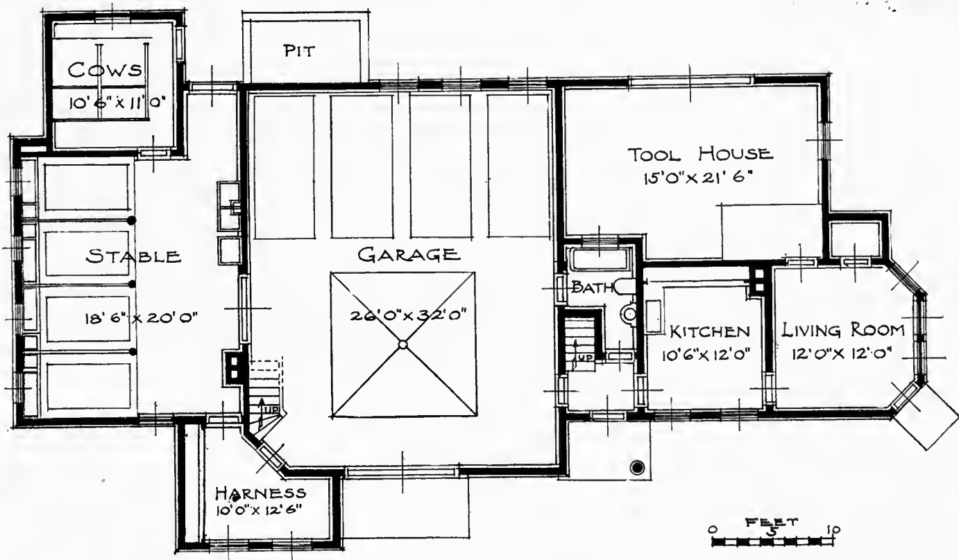
STABLE AND GARAGE AT WILLOUGHBY, OHIO
