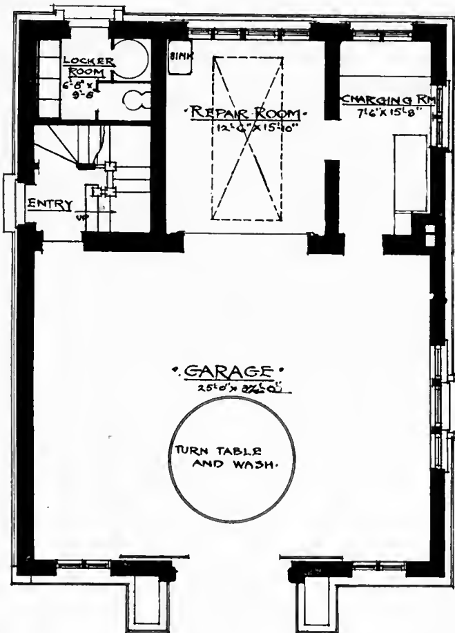
A CHICAGO GARAGE
