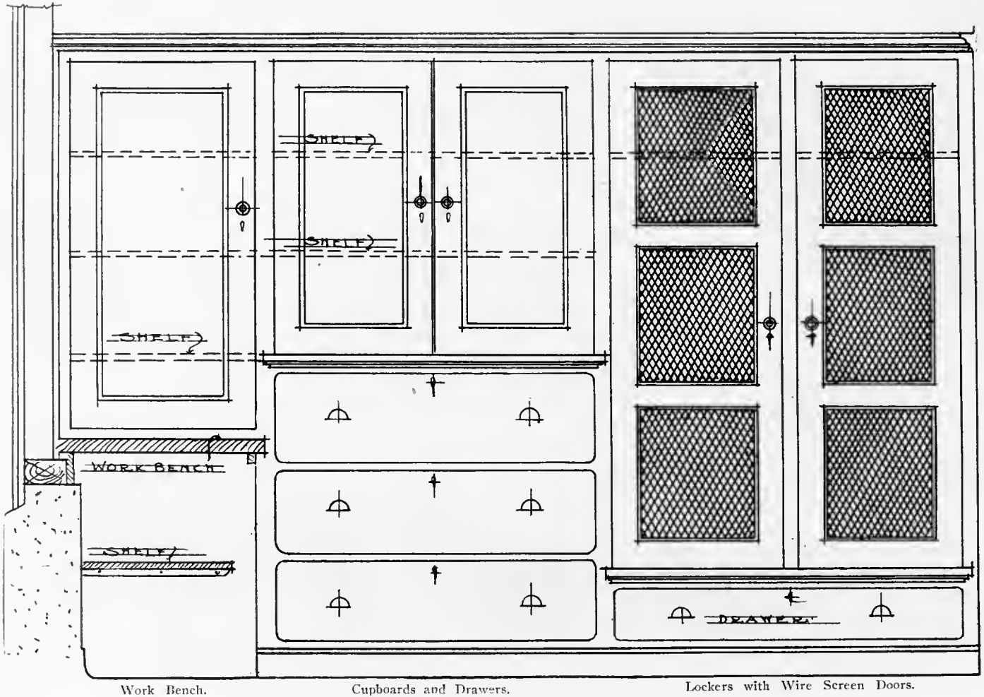
DETAIL OF LOCKERS IN SHOP Kilham & Hopkins, Architects
