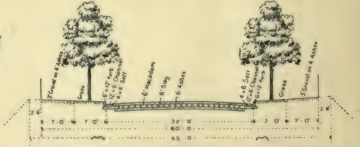
60 feet roadway on an embankment showing 2 ft. 6 ins. allowance on either side beyond the boundary lines.
