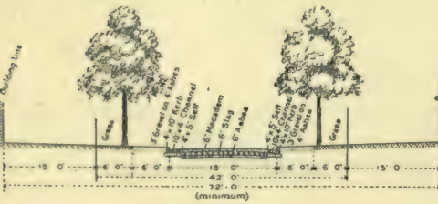
42 feet roadway with 18 feet metalled but a minimum of 72 feet between the building lines.
