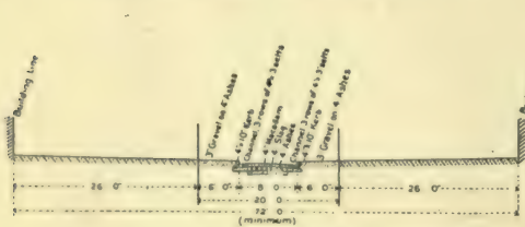
20 feet roadway with 8 feet metalled but a minimum of 72 feet between the building lines.
