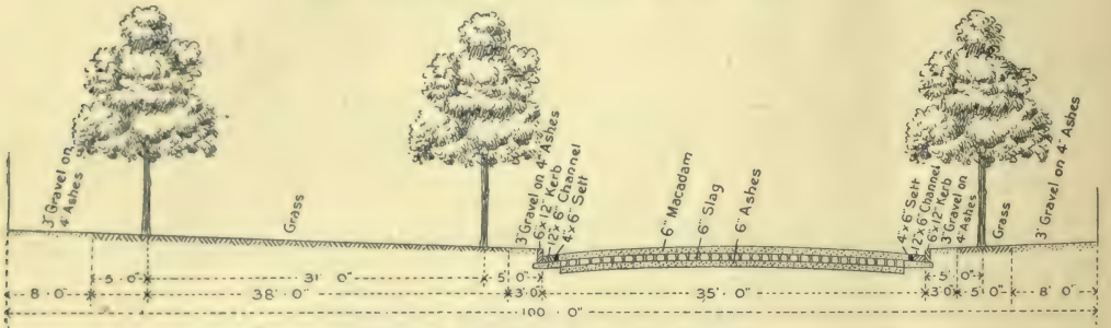
80 feet roadway, with 35 feet metalled and 22 feet devoted to grass margins.
