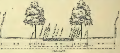
36 feet roadway with 18 feet metalled but a minimum of 72 feet between the building lines.
