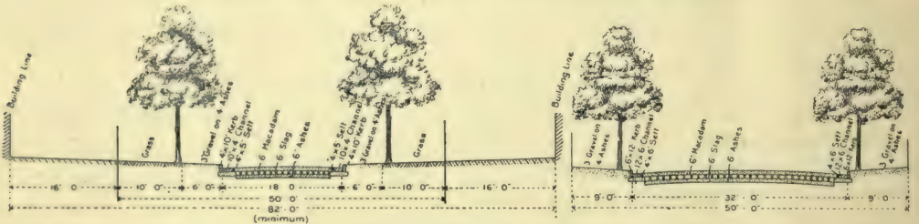
50 feet roadway with 18 feet metalled but a minimum of 82 feet between the buildings
