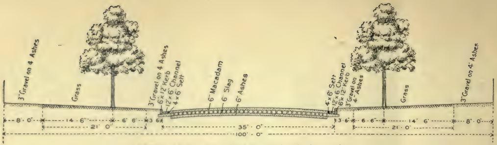
Main road 100 feet wide, metalled only for 35 feet.
