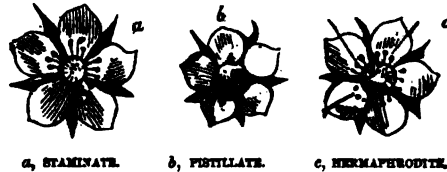
a, STAMINATE.
