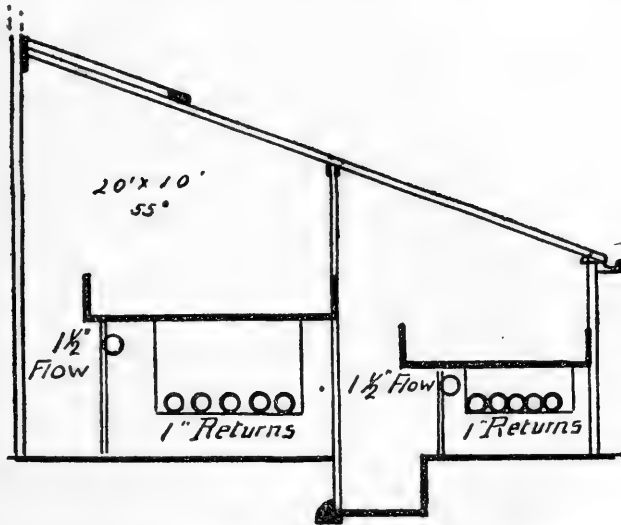
Fig. 8—Hot water is undoubtedly the most satisfactory method of heating the small greenhouse. The diagram shows a 1\frac{1}{2} -inch supply pipe leading out from the boiler, with 1-inch returns under the benches, making a satisfactory system for the lean-to type described in detail in the previous chapter.
