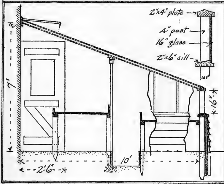
Fig. 3—A sectional view of a two-bench, 10 x 20 ft. house built against the dwelling wall. If possible it would be well to gain a steeper slope for the glass and better headroom. The detail in the upper right hand corner shows, at larger scale, the plate and front lights, indicated just below in the main section.
