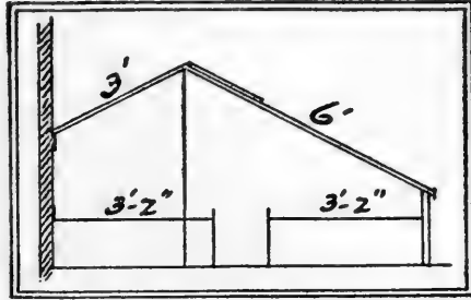
Fig. 4—A simple form of lean-to greenhouse where there is an available sheltering wall but with first-story windows. The inner slope or valley should be drained
