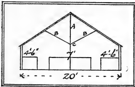
Fig. 6 — The regular even-span type. A indicates a row of pipe standards; BB, braces from these to the purlins. There is a fitting made for the junction C.
