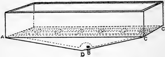
Fig. 1.—Box for plants. AC—false zinc bottom; AB, CB—slanting bottom to drain water out at hole B.
