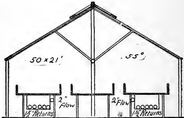
Fig. 9—For the larger greenhouse of the isolated double-slope type, 21 x 50 feet in size, a 2-inch supply pipe, with five 1½-inch returns under the outer benches, will secure a temperature of 55 degrees.
