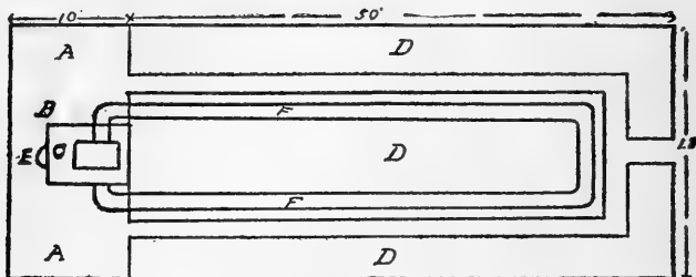
Fig. 7 —The best arrangement for heating a greenhouse by hot air, is to run a brick or cement flue from the furnace around under the benches and into the chimney over the fire. AA—storage space; B—furnace; C—chimney; DDD—benches; E—furnace door.
