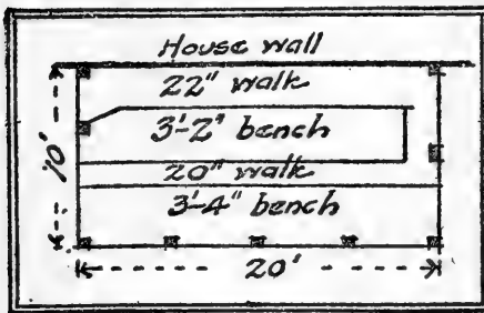
Fig. 2—Floor plan of the lean-to type of greenhouse shown in section on the opposite page.
