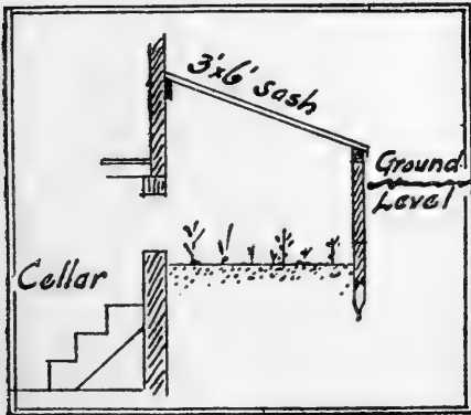
Fig. 5—The simplest of all "greenhouses," which is in reality little more than a deep coldframe with an opening into the cellar
