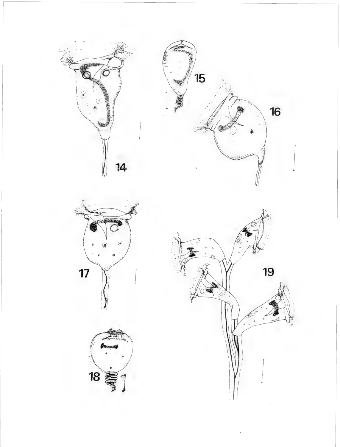
FIGURES 14-19. 14. Vorticella picta , 15. contracted zooid of V. picta , 16. Vorticella pulchella , 17. Vorticella rotunda , 18. contracted zooid of V. rotunda , 19. Zoothamnium ramosissimum . Scales: 10 \mu m (Figs. 14, 15, 16, 17, 18), 20 \mu m (Fig. 19).
