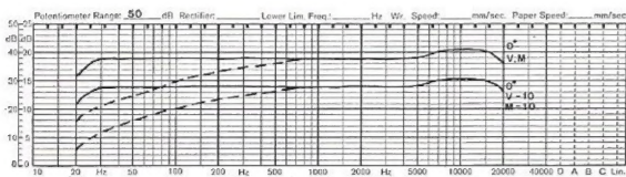
Typical frequency response curve of VM-40/12, VM-40
