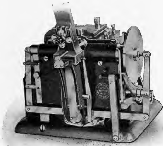
FIG. 46. The Waltham Automatic Pinion Cutter, with Magazine and Self-feeding Mechanism.
