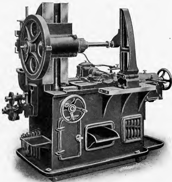
FIG. 30. The Reinecker Automatic Spur Gear Cutting Machine.
