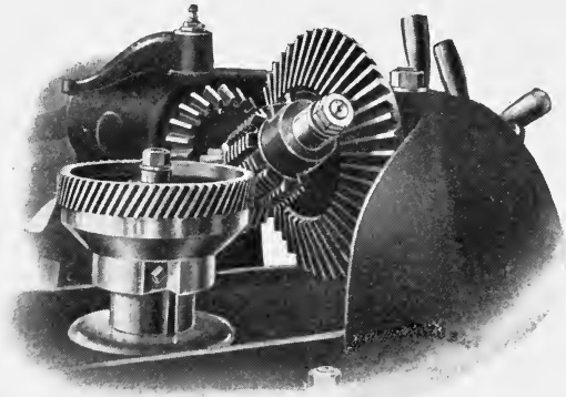
FIG. 124. Grant-Lees Machine hobbing a Helical Gear.
