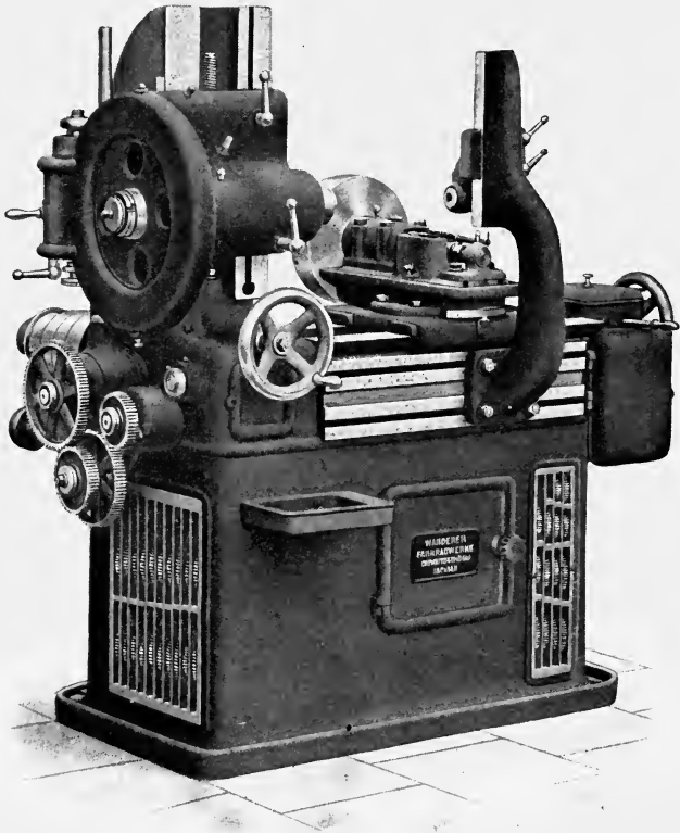
FIG. 61. The Wanderer Spur Gear Hobbing Machine.
