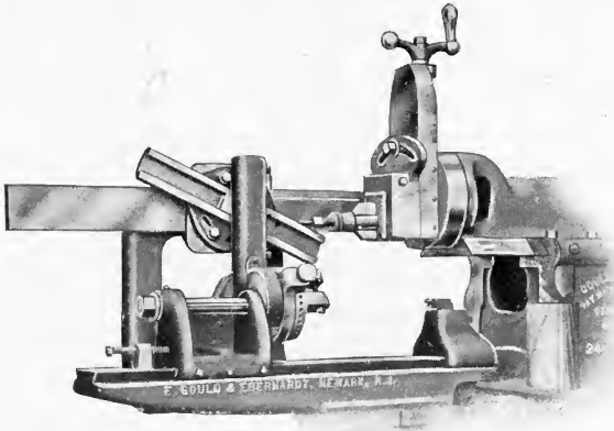
FIG. 96. Helical Attachment for Gould & Eberhardt Shaper, in which the Lead of the Helix is obtained by the adjustment of a Swiveling Guide Bar.
