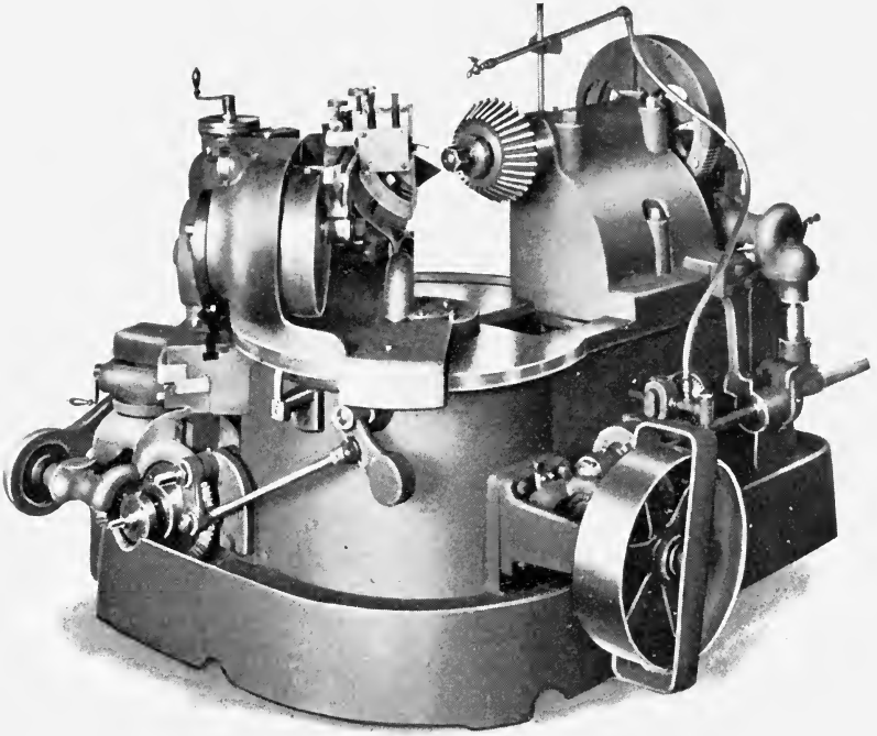
FIG. 179. Gleason Templet-controlled Bevel Gear Planing Machine.
