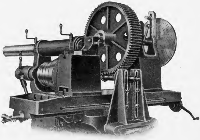
FIG. 13. Attachments for cutting Gears of Large Diameter on Cincinnati Milling Machines.
