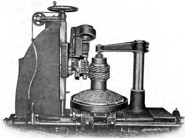
FIG. 119. Gould & Eberhardt Machine cutting Spiral Gears of Large Helix Angle.
