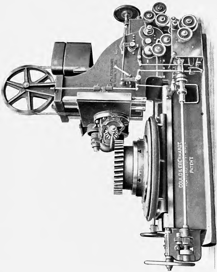
FIG. 110. Automatic Helical Gear-Cutting Machine, made by Gould & Eberhardt.
