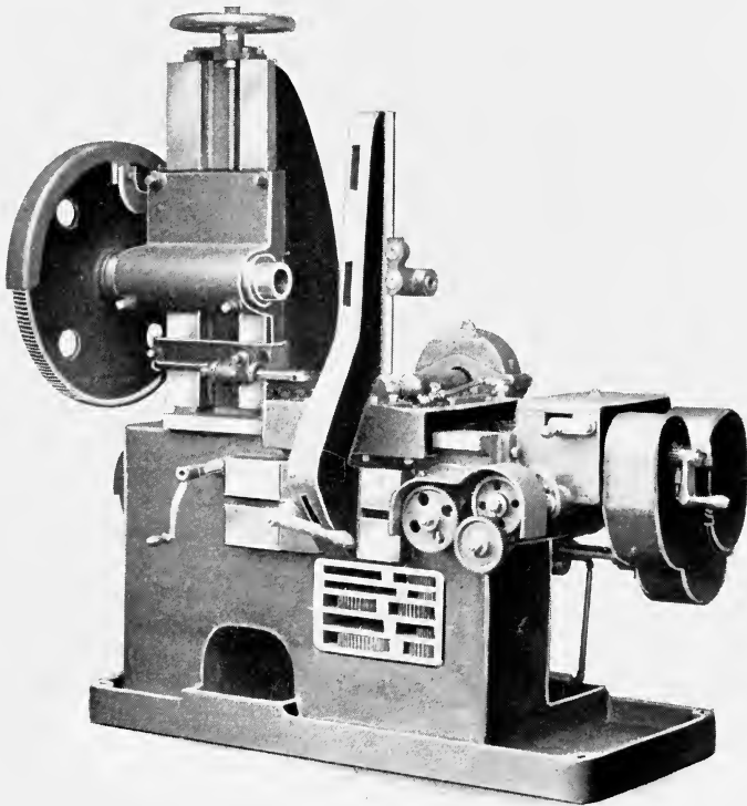
FIG. 23. Automatic Gear-Cutting Machine made by Cincinnati Gear Cutting Machine Company.
