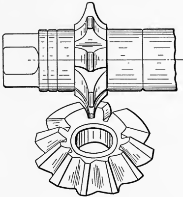
FIG. 160. Shaping the Teeth of a Bevel Gear by the Formed Cutter Process.
