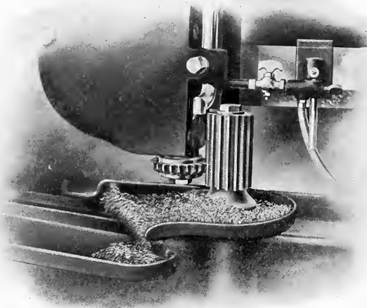
FIG. 55. Detailed View of the Fellows Gear Shaper in Action; see also Figs. 79 and 94.
