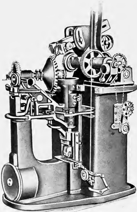
FIG. 188. The Rice Bevel Gear Milling Machine, which forms the Teeth from a Master Gear on the Templet Principle.
