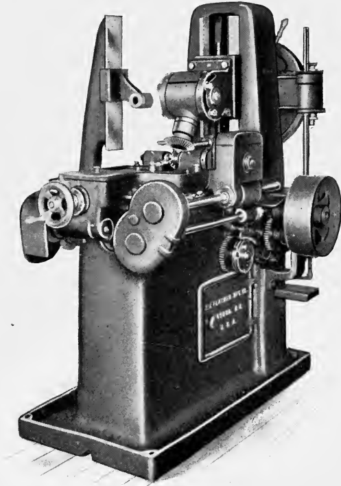
FIG. 170. An Attachment to the Fletcher Automatic Spur Gear Cutter for the cutting of Bevel Gears.
