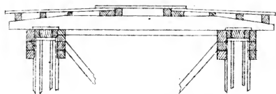
CROSS SECTION.
