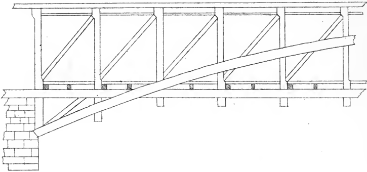
CROSS SECTION.
