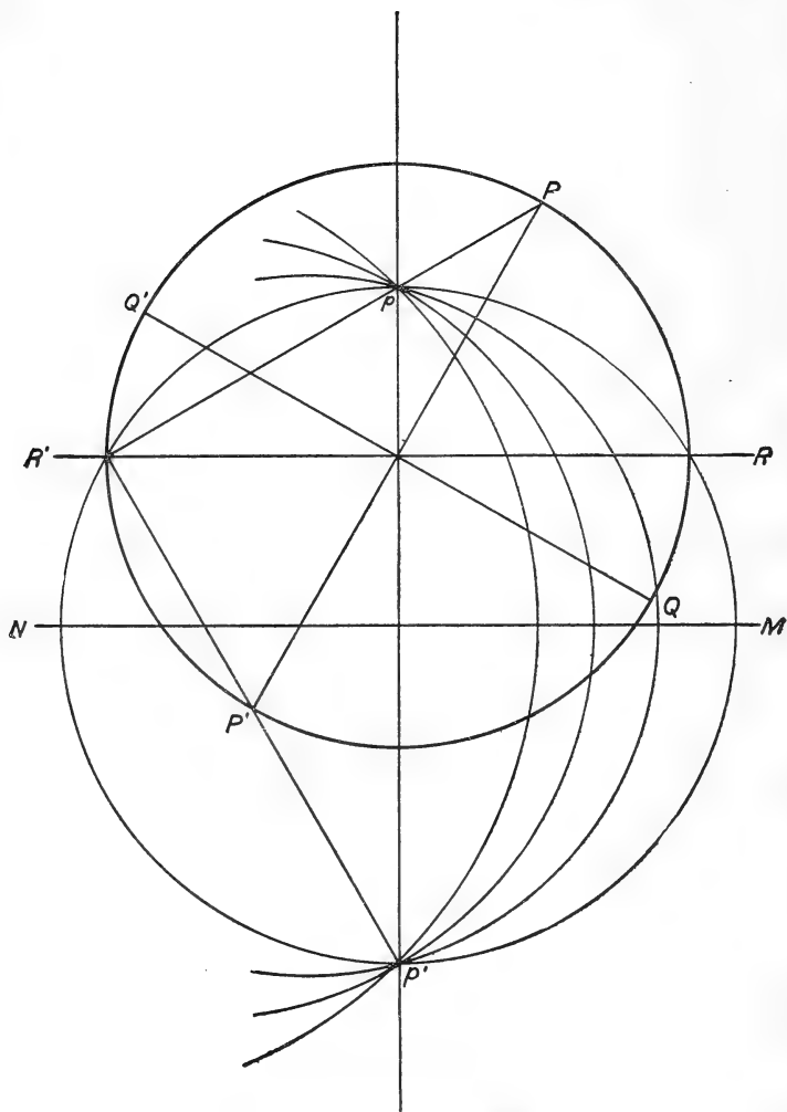
FIG. 32.—Cayley's principle.
