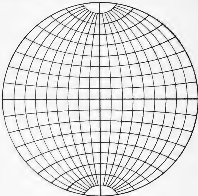
FIG. 37.—Nicolosi's projection or globular projection.
