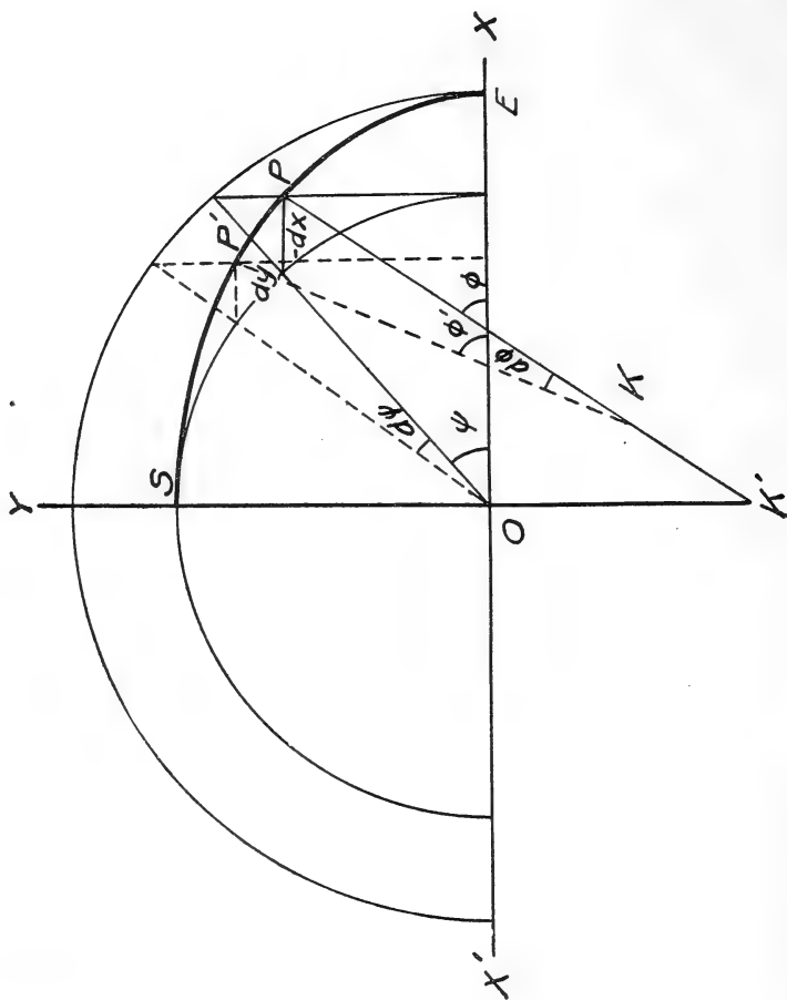
FIG. 1.—Generating ellipse with the radii of curvature of the earth.
