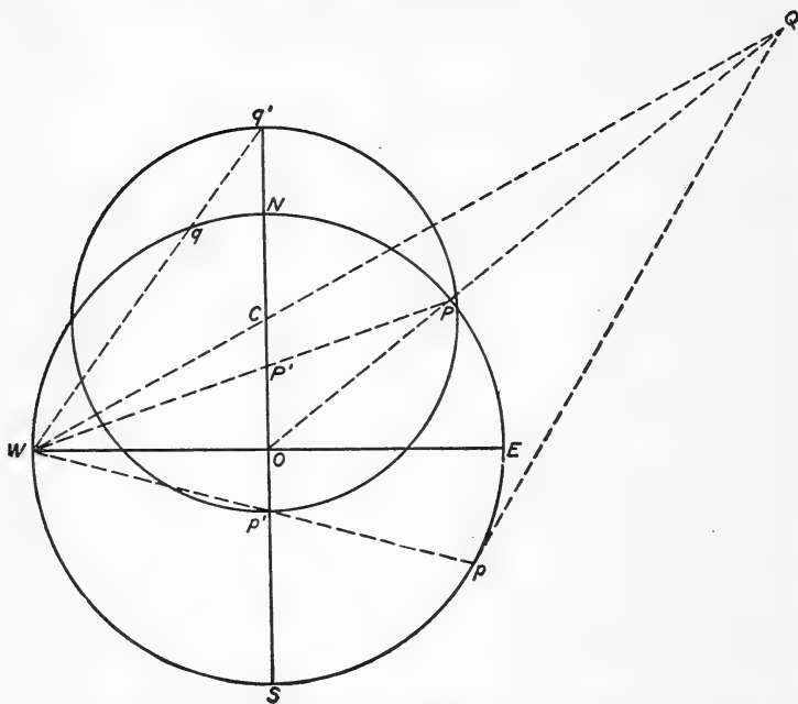
FIG. 16.—Projection of a circle with given projection of pole and given polar distance on stereographic projection.
