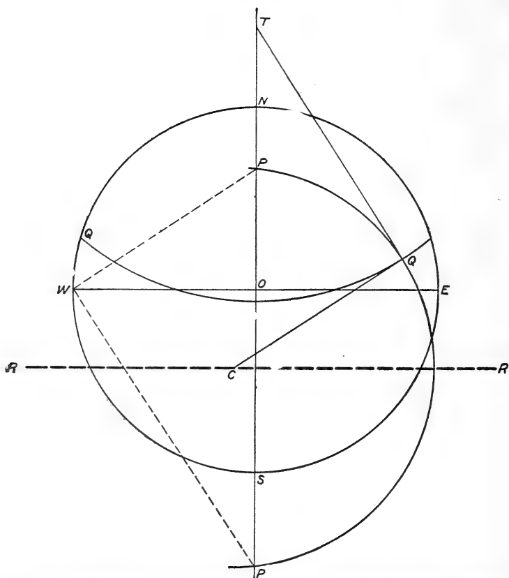
FIG. 28.—Projection of the meridian and parallel through a given point on stereographic projection.
