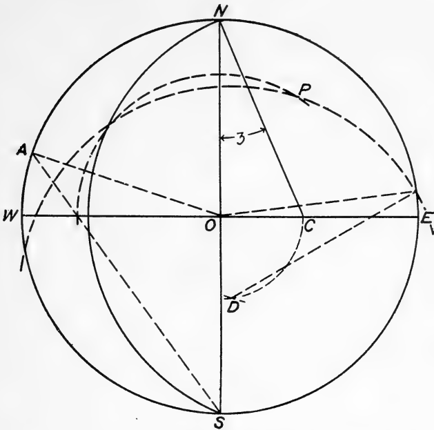
FIG. 26.—Projection of great circle with given inclination to the primitive plane on stereographic projection.
