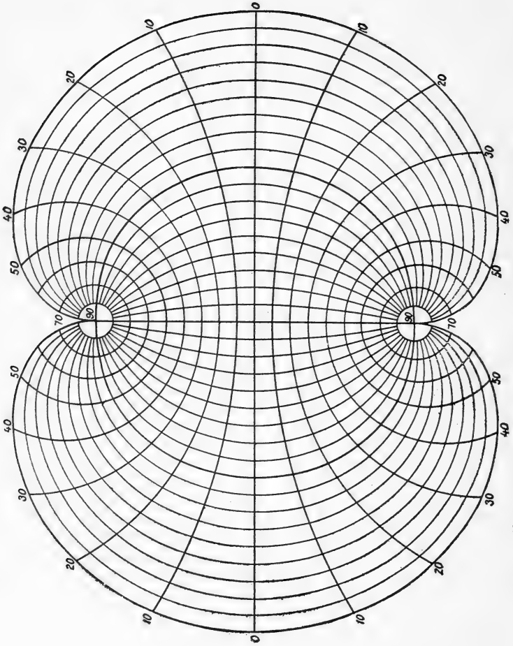
FIG. 40.—Ordinary or American polyconic projection of the entire sphere.
