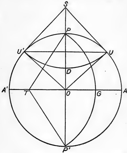
FIG. 35.—Geometrical relations of atractozonic projections.
