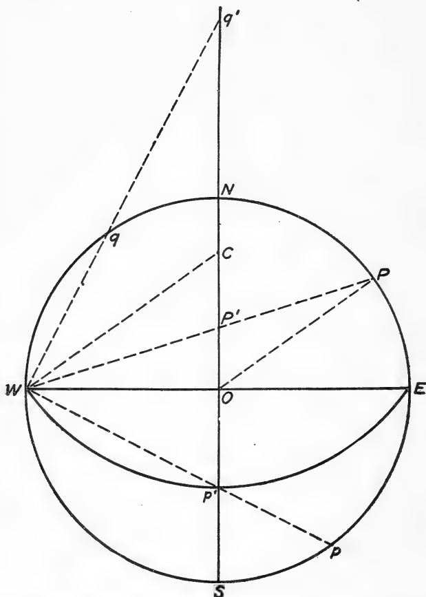
FIG. 18.—Projection of a great circle with given pole projection on stereographic projection.
