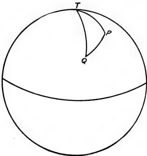
FIG. 9.—Transformation triangle for stereographic horizon projection.
