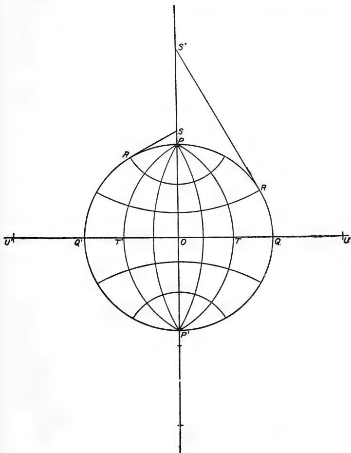
FIG. 8.—Construction of stereographic meridian projection.
