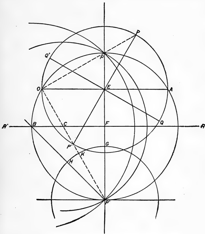
FIG. 13.—Construction of meridians on stereographic horizon projection.
