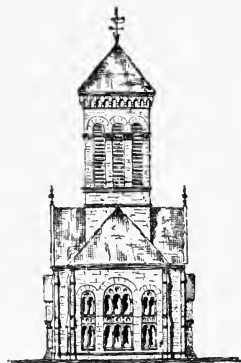
FIG. 82.—SIDE ELEVATION.
