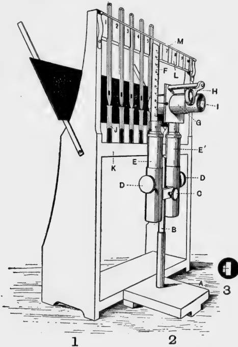
FIG. 108.—Apparatus for quantitative estimation of specific precipitation (Nuttall and Inchley, in "Journal of Hygiene.")
