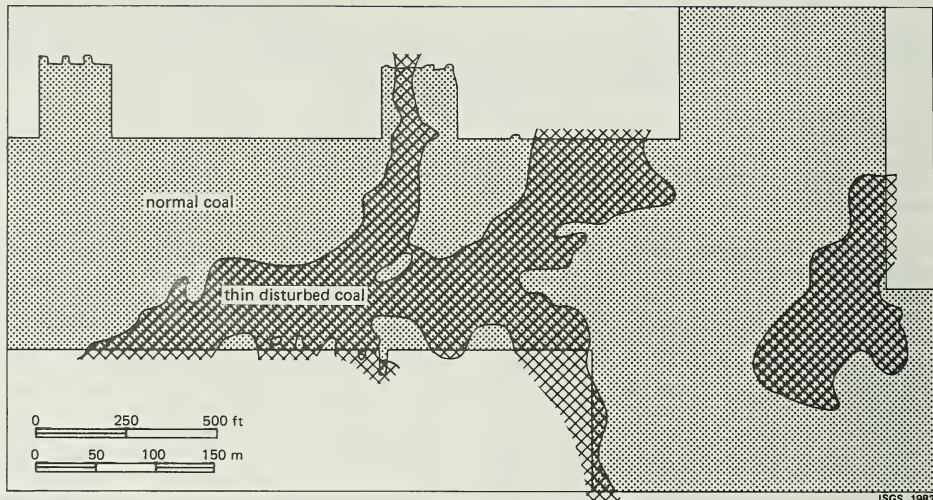
Figure 28 Thin and disturbed coal associated with limestone rolls at the Peabody River King underground mine in St. Clair County. The pattern suggests a drainage system of small streams in the coal-forming swamp.
