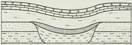
c. More deposits covered the channel. The channel-fill materials compacted more than the surrounding materials, so a trough developed above the buried channel.
