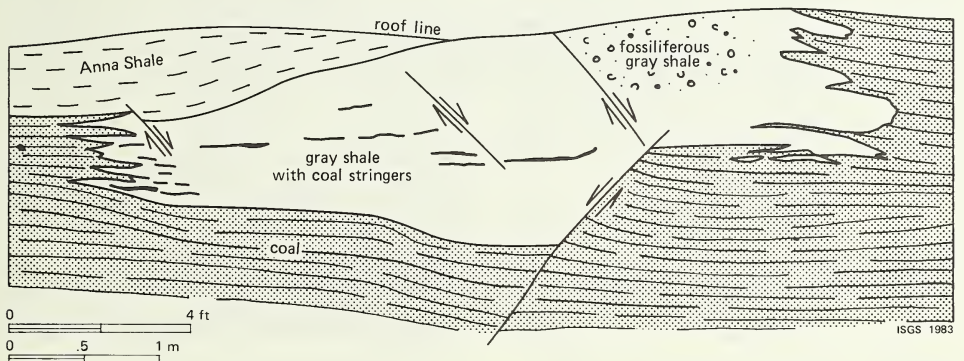
Figure 25 Field sketches of rolls in Old Ben Mine No. 24. Rolls are filled with gray shale but overlie by black (Anna) shale.
