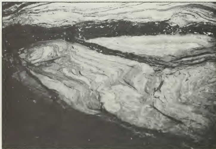
Figure 24b Close view of another sandstone-filled roll at Inland Mine No. 1. Note the strongly contorted laminations in the sandstone, perhaps a result of sediments slumping while still soft.
