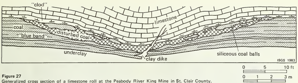
Figure 27 Generalized cross section of a limestone roll at the Peabody River King Mine in St. Clair County.
