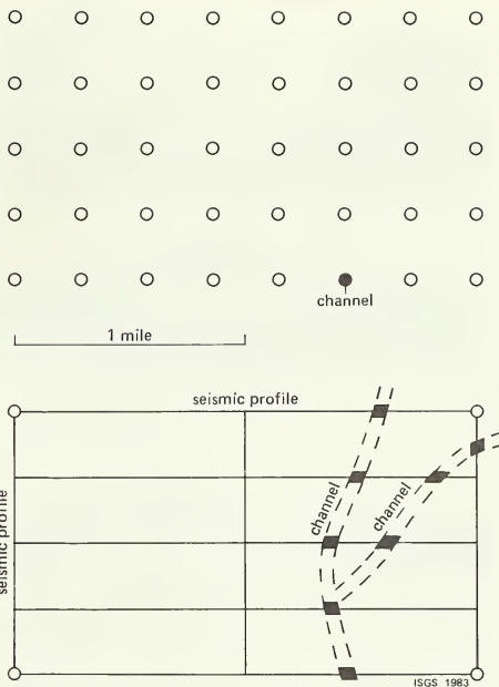
Figure 13 Locating channels with high-resolution seismic profiling (modified from Daly, 1979). The upper grid represents 40 exploratory drill holes. Although one hole penetrated a channel, the available data gave no clues to the extent or trend of the channel. In the lower diagram, 4 drill holes and 8 seismic profiles provide an accurate pattern of the cutouts.
