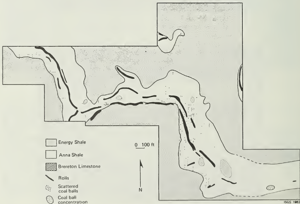
Figure 26 Lithology of the immediate roof, rolls, and coal balls in part of Old Ben Mine No. 24 in Franklin County. Anna Shale occurs in elongate belts suggestive of channels (perhaps tidal channels). Rolls occur only under Anna Shale and run parallel with the border between Anna and Energy Shales. Coal balls occur only under marine roof (from Bauer and DeMaris, 1982).
