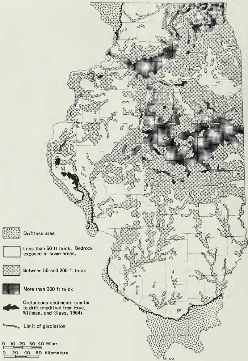
Figure 2 Generalized thickness of glacial drift in Illinois (from Piskin and Bergstrom, 1975).
