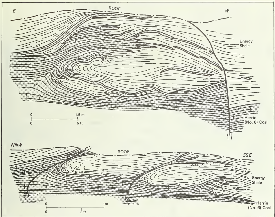
Figure 21 Field sketches of rolls filled with gray shale in the Herrin (No. 6) Coal (from Krausse et al., 1979).
