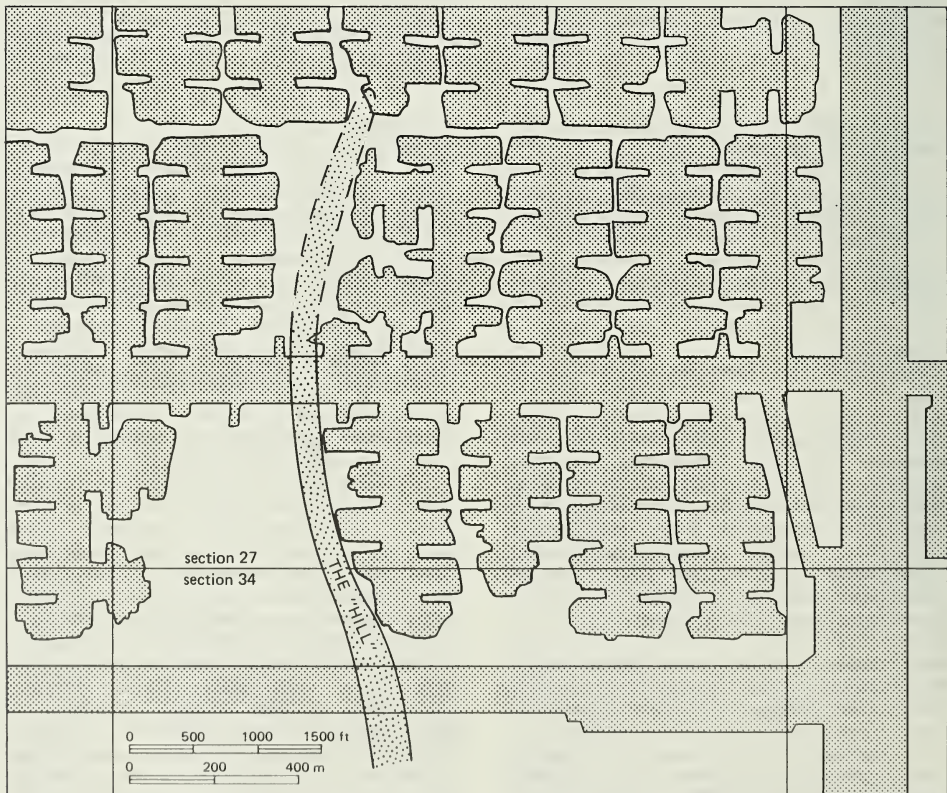
Figure 40 Part of the workings of Peabody Mine No. 10, showing the hill.
