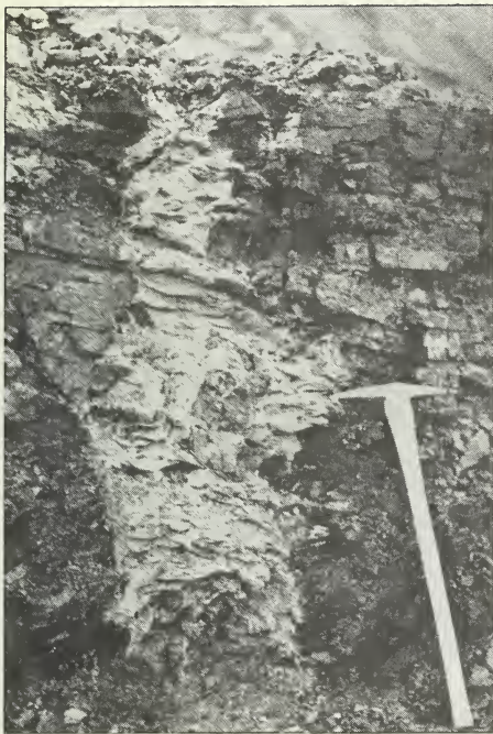
Figure 31 Clay dikes or horsebacks: (left) in the Springfield (No. 5) Coal at a surface mine in west-central Illinois; (right) in the Springfield Coal and overlying black shale at the abandoned El-Ben Mine in Logan County. The dike at the El-Ben Mine branches upward into myriad, small fissures, and veinlets that severely inhibit roof stability (photo shows Ronald Kern, formerly of the ISGS). (Photos by H. H. Damberger.)
