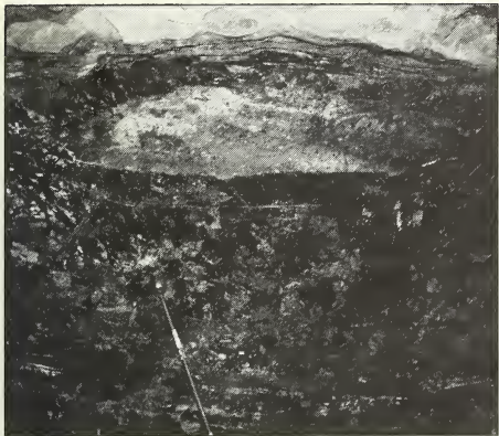
Figure 38 Coal ball (about 3 ft long and 1 ft thick) near top of the Herrin (No. 6) Coal in the Orient Mine No. 4, Freeman United Coal Company, Williamson County. The roof is limestone on a thin base of shale.
