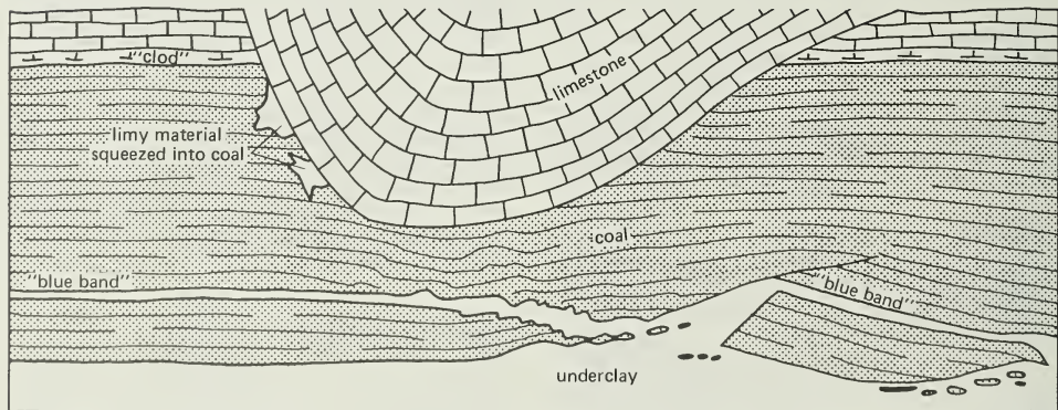
Figure 29 Field sketch of a limestone roll at Peabody Camp Mine No. 11 in Union County, Kentucky.
