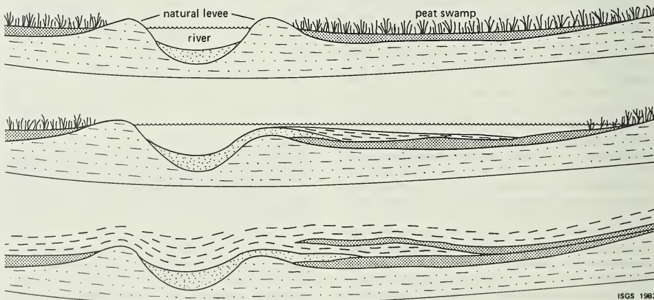
Figure 14 Split coal may form in three ways.
