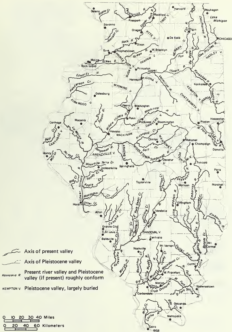
Figure 1 Pleistocene valleys or channels in Illinois, compared with present drainage systems (from Piskin and Bergstrom, 1975).
