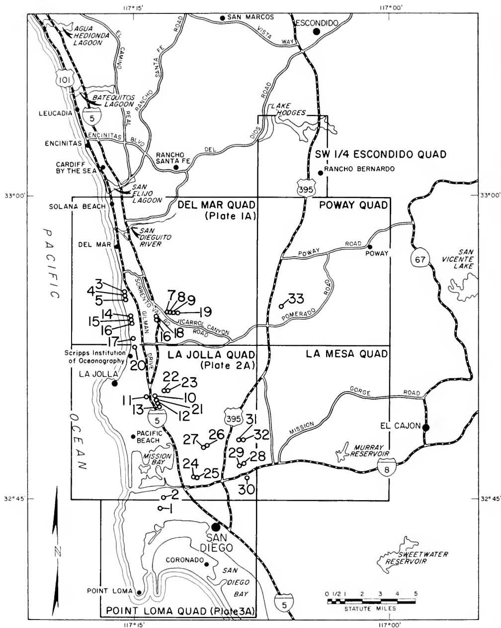
Figure 7. Index map of fossil mollusk localities. (See plates 1A-3A and plate 2B (Kennedy and Peterson, 1975) for detailed locations.)
