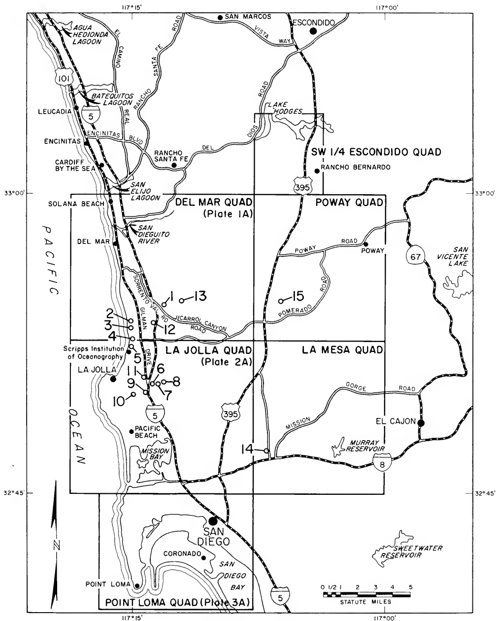
Figure 8. Index map of fossil calcareous nannoplankton localities. (See plates 1A, 2A and plate 2B, 3B (Kennedy and Peterson, 1975) for detailed locations.)
