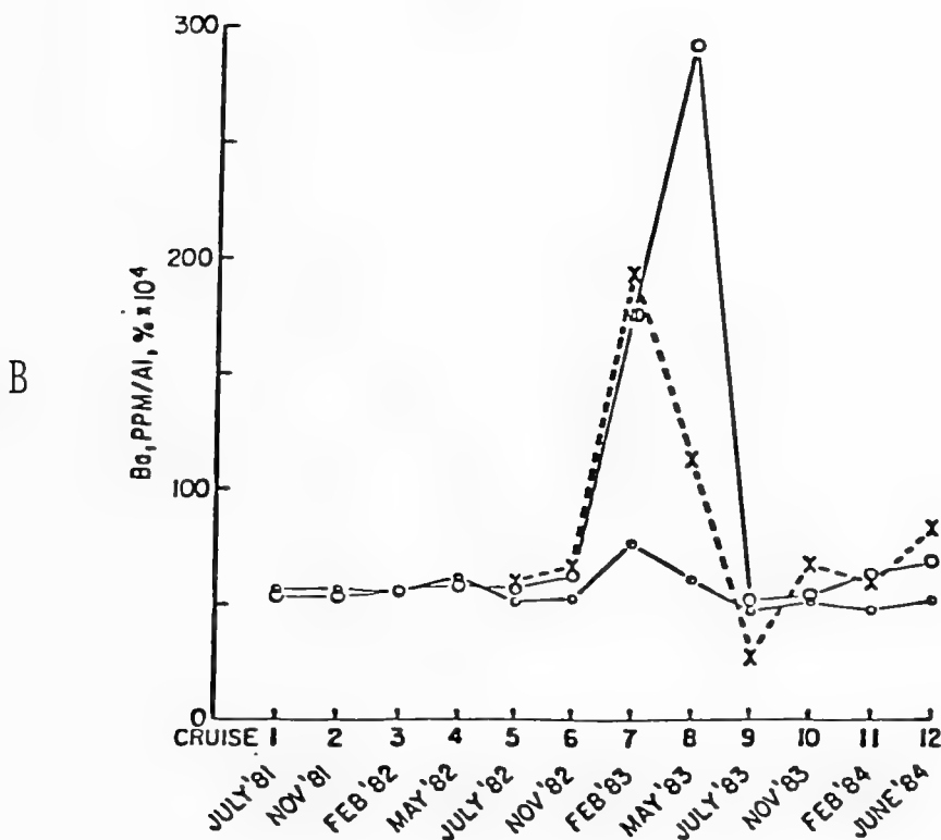
FIGURE 9A and 9B. Concentrations of barium (9A) and the barium to aluminum ratio (9B) in the fine fraction of sediment blends on different sampling occasions at stations 2 (X), 3 (O), 10 (□), and 12 (O).
