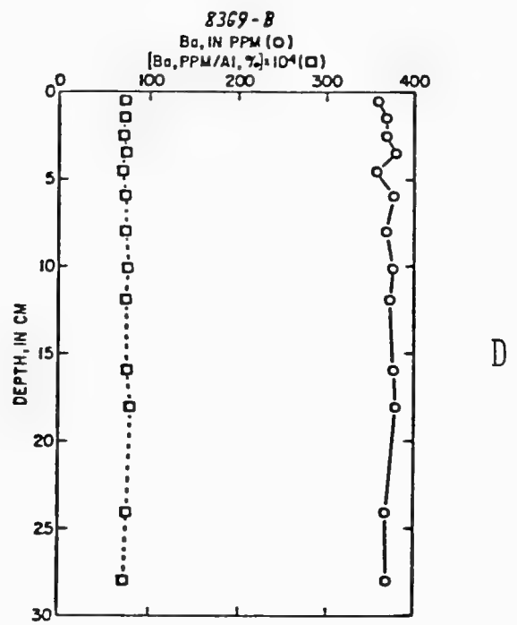
FIGURE 15 A-D. Distributions of barium and the barium to aluminum ratio with sediment depth. Analyses were performed on the fine fraction of sediment. Stations 2 and 3 were sampled with a grab sampler. Samples OC140-8B and 8369-3 were collected with a hydraulically damped gravity corer and a box corer, respectively.
