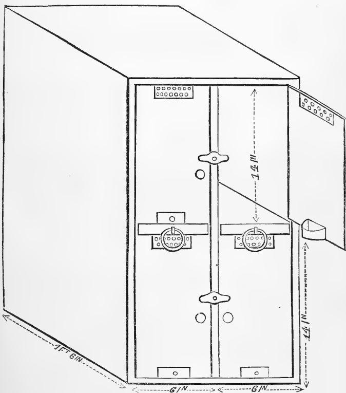
Fig. 20. Perspective Elevation of Improved Fattening Pens for Cramping Poultry.
