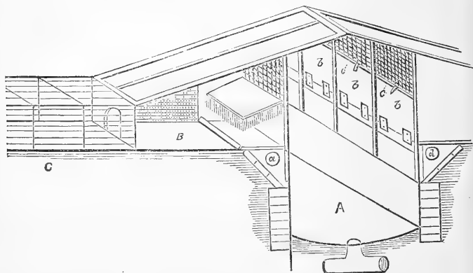
Fig. 18. Artificial Rearing Home—Perspective Section.
