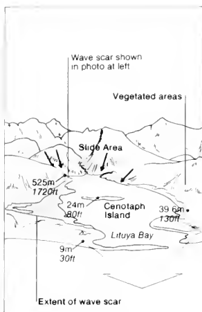
A 1958 earthquake triggered a landslide at Lituya Bay's upper end. The slide created a wave that denuded the promontory facing it (shown at the left in the photo of Lituya Glacier) to an altitude of 525 meters (1,720 feet). Three boats were in the bay. The island protected one. A second washed over the sandspit at the bay's mouth and into the ocean. The third was destroyed. The drawing shows the extent of denuded shorelines.
