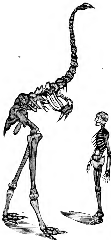
SKELETON OF A MAN AND THAT OF A DINORNIS SHOWING COMPARATIVE SIZE.
