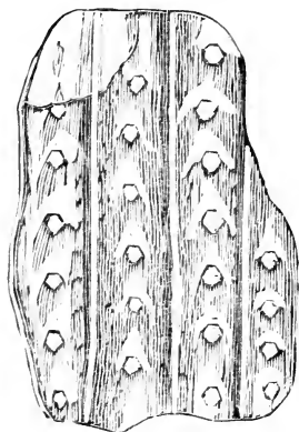
SPECIMEN OF BARK FROM A NOVA SCOTIA COAL MINE.
