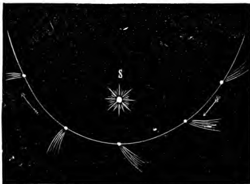
COMET PASSING ROUND THE SUN (ITS PERIHELION).
