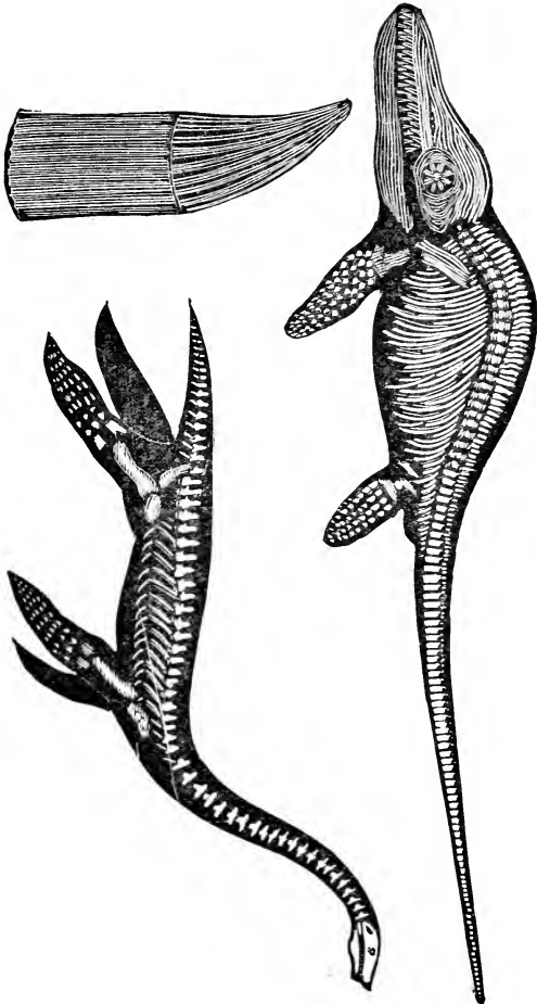
REMAINS OF PLESIOSAURIUS AND MEGALOSAURIUS.
