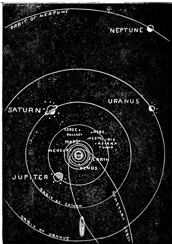
SOLAR SYSTEM.
