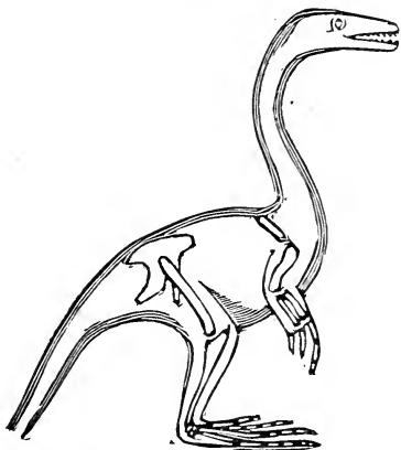
BIRD-LIKE REPTILE DISCOVERED BY DARWIN.
