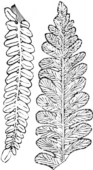
FERNS.
