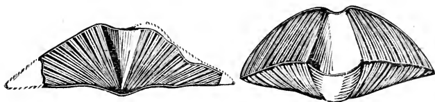
REMAINS OF SHELL FISH.
