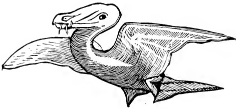
REPTILIAN BIRD BY HUXLEY.
