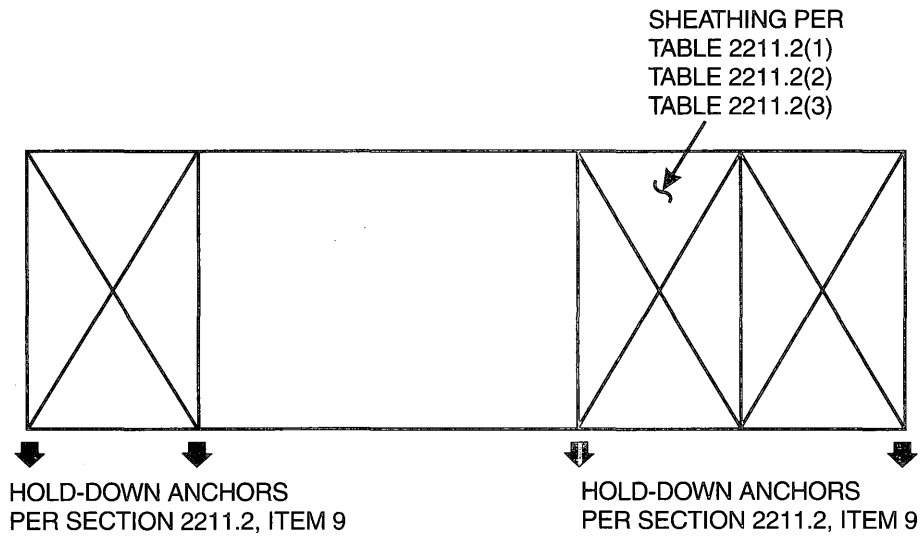
TYPE I SHEAR WALL
