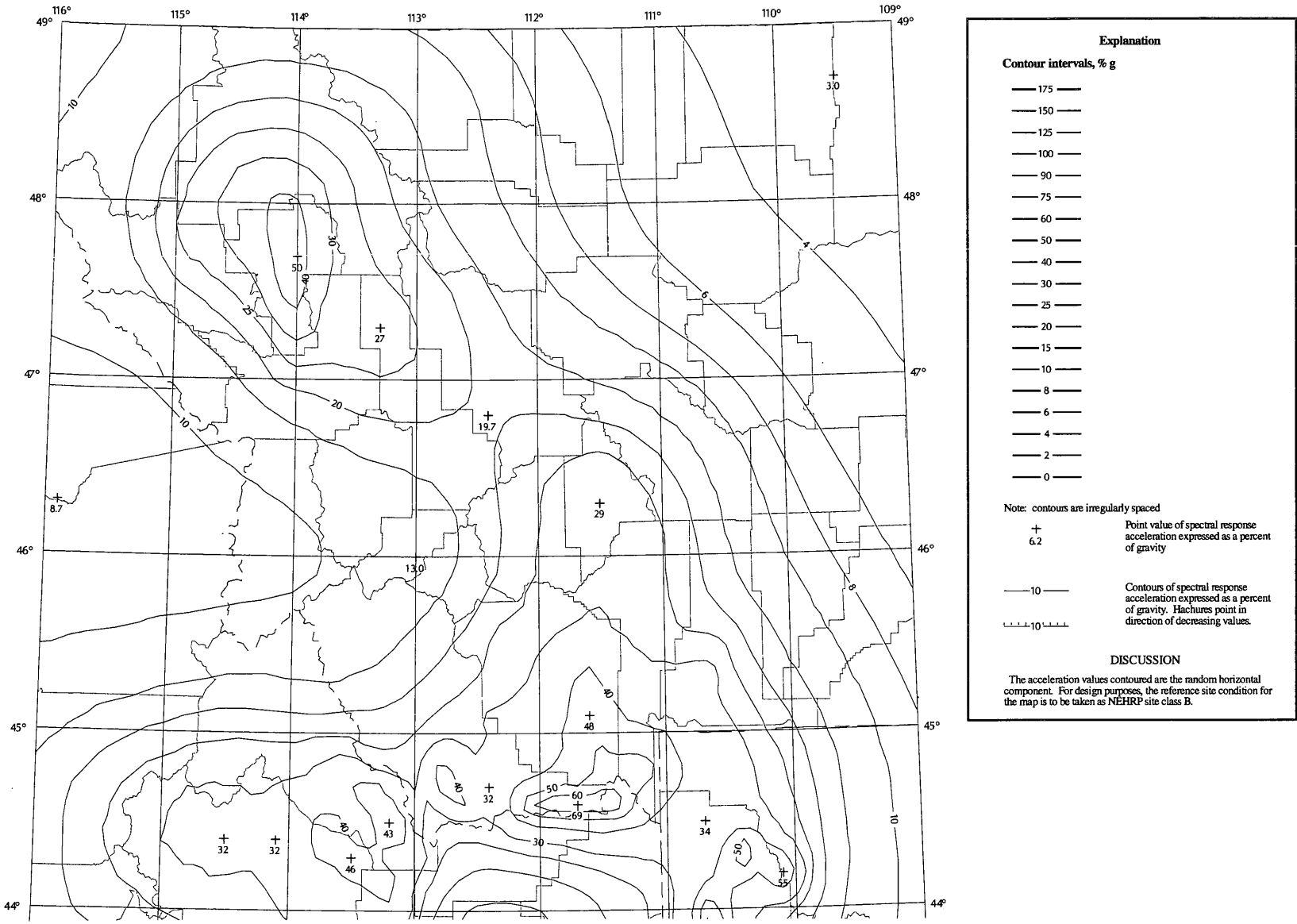
FIGURE 1615(6) MAXIMUM CONSIDERED EARTHQUAKE GROUND MOTION FOR REGION 2 OF 1.0 SEC SPECTRAL RESPONSE ACCELERATION (5 PERCENT OF CRITICAL DAMPING), SITE CLASS B
