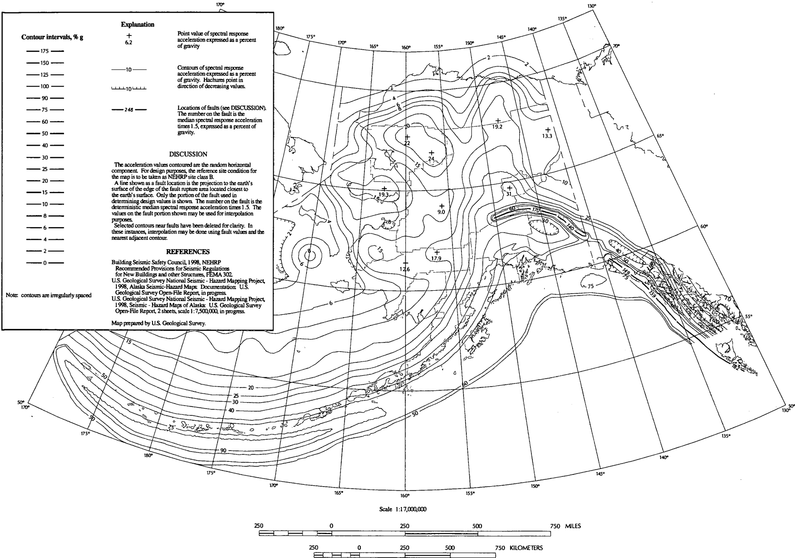
FIGURE 1615(7)—continued MAXIMUM CONSIDERED EARTHQUAKE GROUND MOTION FOR ALASKA OF 1.0 SEC SPECTRAL RESPONSE ACCELERATION (5 PERCENT OF CRITICAL DAMPING), SITE CLASS B
