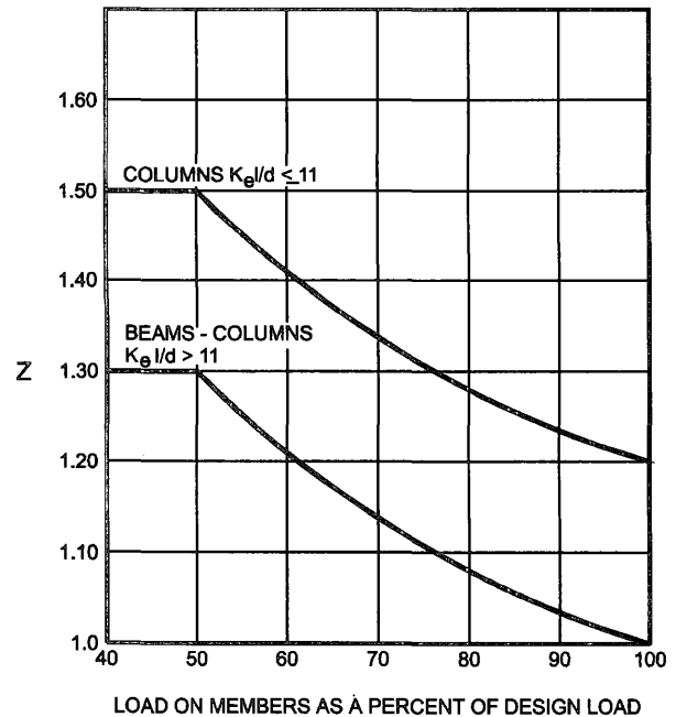
FIGURE 721.6.3(1) LOAD FIGURE
