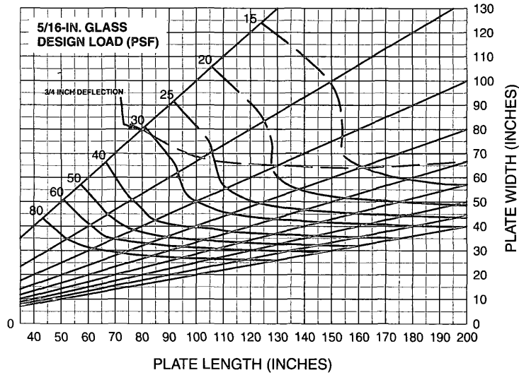
FIGURE 2404(7) a, b, c, d, e, f MAXIMUM ALLOWABLE LOAD FOR VERTICAL AND SLOPED RECTANGULAR GLASS SUPPORTED ON ALL EDGES
