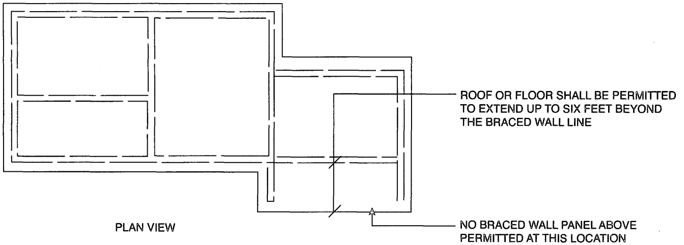
FIGURE 2308.12.6(1) BRACED WALL PANELS OUT OF PLANE
