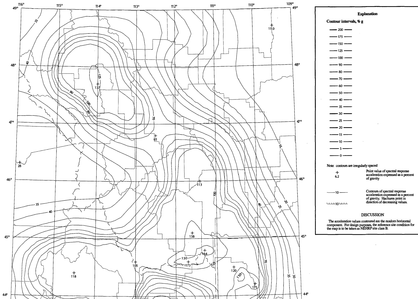
FIGURE 1615(5) MAXIMUM CONSIDERED EARTHQUAKE GROUND MOTION FOR REGION 2 OF 0.2 SEC SPECTRAL RESPONSE ACCELERATION (5 PERCENT OF CRITICAL DAMPING), SITE CLASS B
