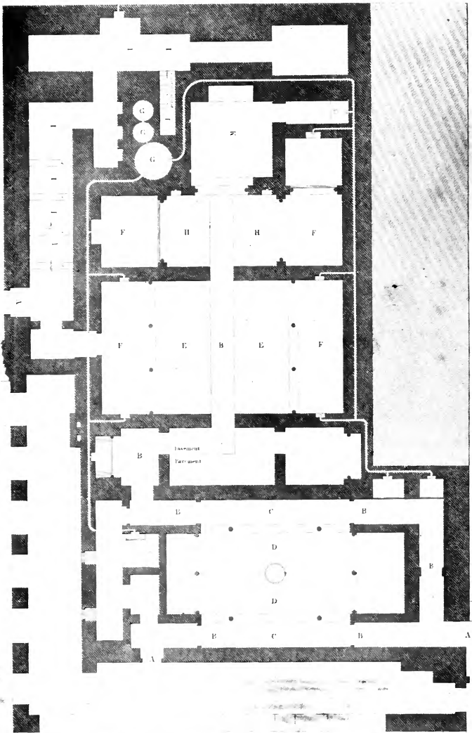
A SECTION PLAN OF THE BATHS, IN THE ALHAMBRA.
