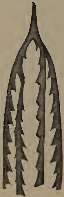
Fig. 55 Tetragraptus pendens Elles. Enlargement of proximal portion of rhabdosome to show the character of sicula and thecae. Deep kill. \times 4.5
