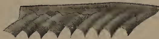
Fig. 57 Tetragraptus serra Brongniart sp. Fragment of branch. Shows the form and inclination of the thecae; and the thick dorsal wall of the coenosarcal canal. Deep kill. x4.8
