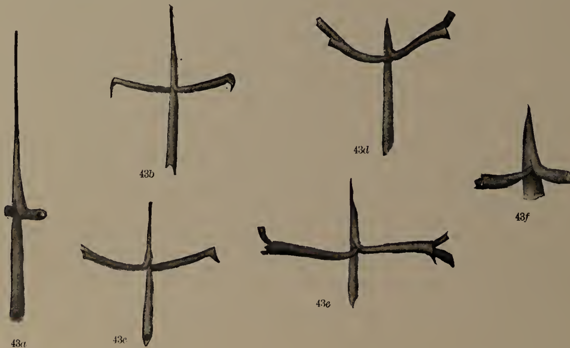
Fig. 43 Goniograptus geometrieus sp. nov. a Sicula and proximal parts of first two thecae. Shows nema, which has become too thick in the zincograph. \times 8 ; b Growth stage with two thecae, which show apertural processes. \times 7 ; c Like growth stage, where the first theca originates nearer to the apex. \times 7 ; d Growth stage in which the first theca buds extremely close to the apex of the sicula and further dichotomy has set in. Reverse view. \times 7 ; e Young rhabdosome with relatively short or fragmentary sicula. Reverse view. \times 7 ; f Greater enlargement of first dichotomy. \times 21 . Deep kill
