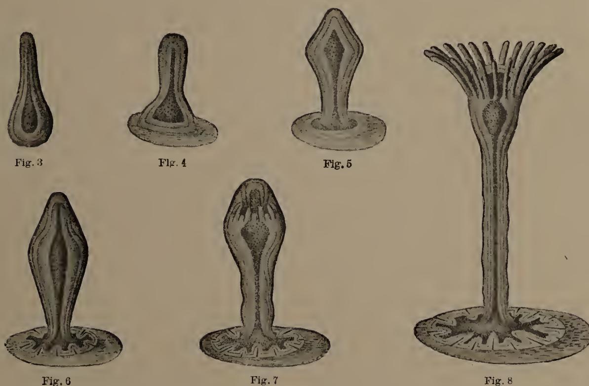
Fig. 3-8 Eudendrium ramosum Linn. Growth stages (Copy from Allman)
