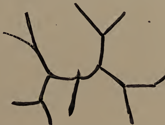
Fig. 44 Goniograptus geometricus sp. nov. Further enlargement of the specimen reproduced on plate 7, figure 12 to show the thecae forming the branches of the first, second and third orders. Deep kill. \times 5.25
