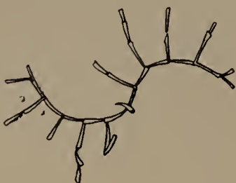
Fig. 15 Coenograptus gracilis Hall sp. x4 (Copy from Ruedemann)
