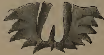
Fig. 60 Tetragraptus similis Hall sp. Proximal portion of rhabdosome. Obverse view. Deep kill. x4.5
