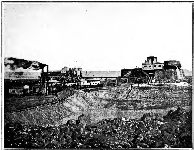
FIG. 10.—Machinery used in preparing the nitrate and iodine.
