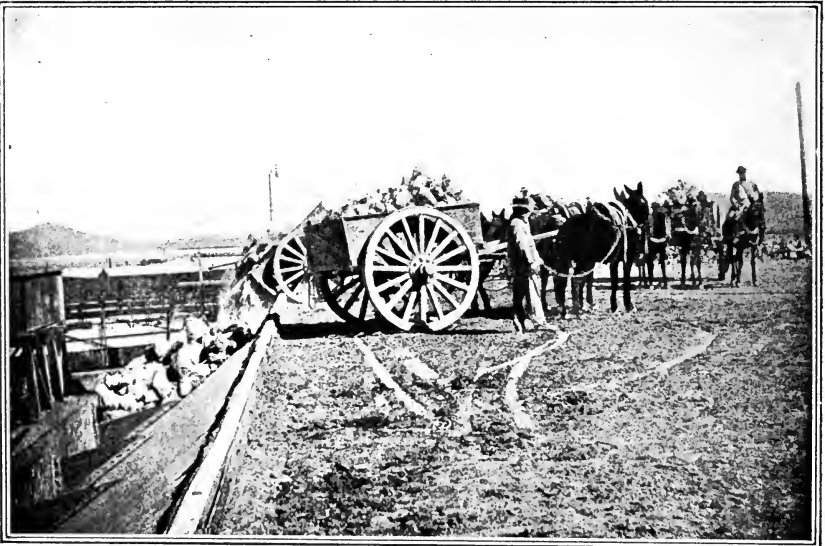
FIG. 8.—Caliche at the crusher.
