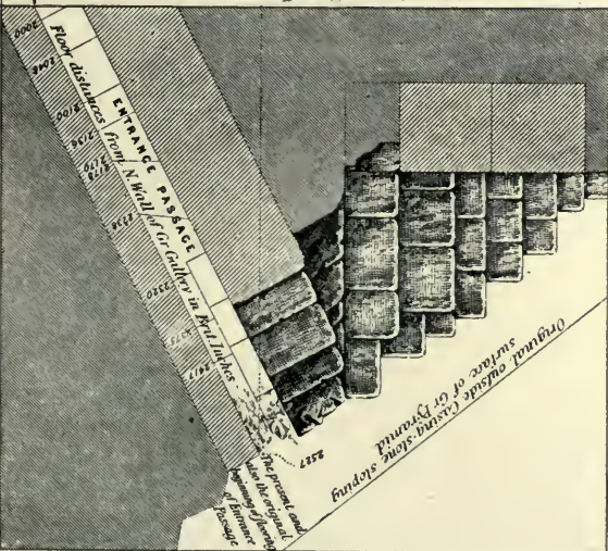
VERTICAL LONGITUDINAL SECTION, looking West. OF THE UPPER, NORTH, END, OR BEGINNING, OF THE ENTRANCE PASSAGE INTO GREAT PYRAMID. SCALE OF BRITISH INCHES. 100 200 300 400 500
