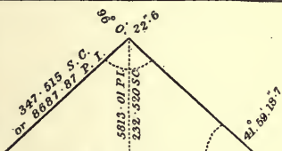
DIAGONAL VERTICAL SECTION OF GREAT PYRAMID.
