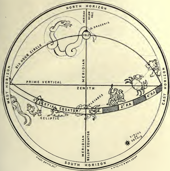
GROUND PLAN OF THE CIRCLES OF THE HEAVENS ABOVE THE GREAT PYRAMID, AT ITS EPOCH OF FOUNDATION AT MIDNIGHT OF AUTUMNAL EQUINOX 2170 B.C. Q. DRACONIS ON MERIDIAN BELOW POLE AT ENTRANCE PASSAGE ANGLE; AND PLEIADES ON MERIDIAN ABOVE POLE IN 0° R.A., OR COINCIDENTLY WITH VERNAL EQUINOX.
