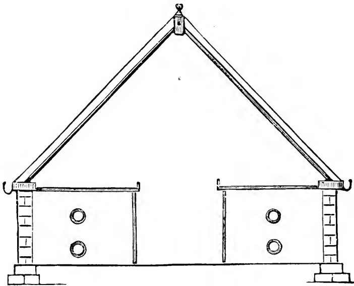
FIG. 11.—SPAN-ROOF HOUSE.
