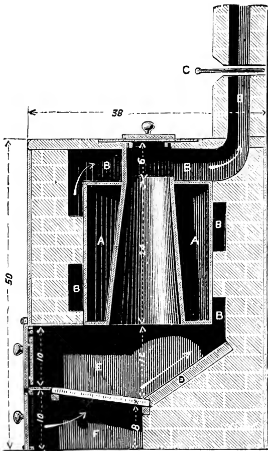
FIG. 18.—PLAIN CONICAL BOILER.
