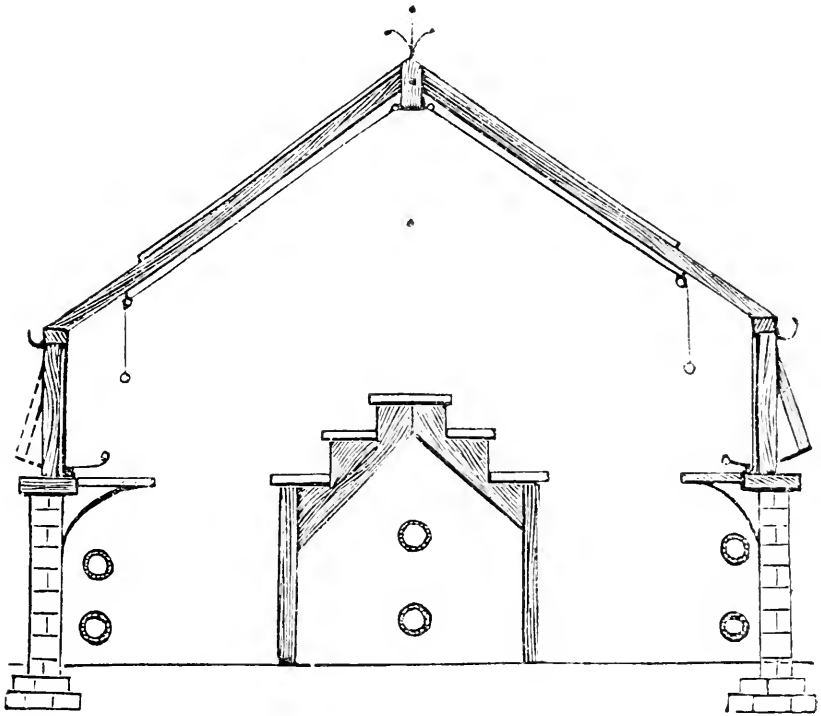
FIG. 12.—SPAN-ROOF HOUSE.
