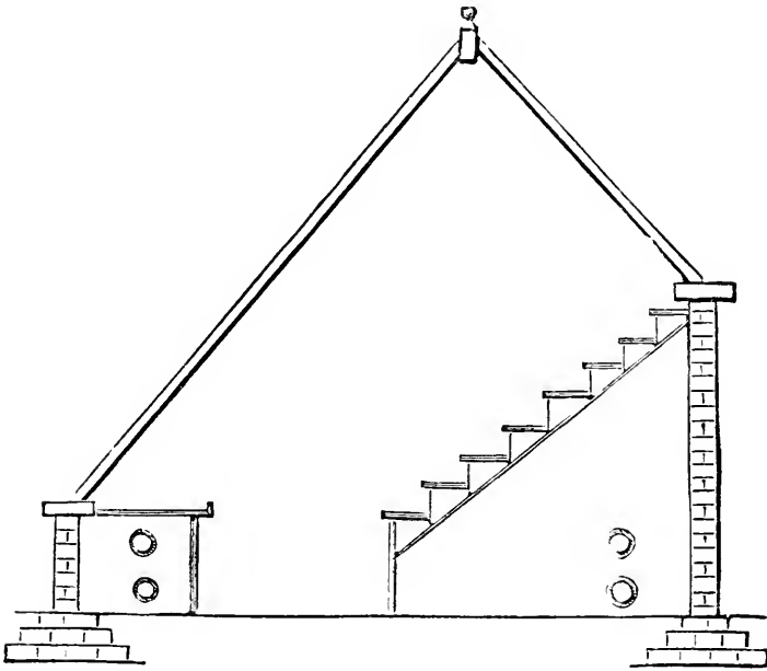
FIG. 10.—HALF-SPAN HOUSE.
