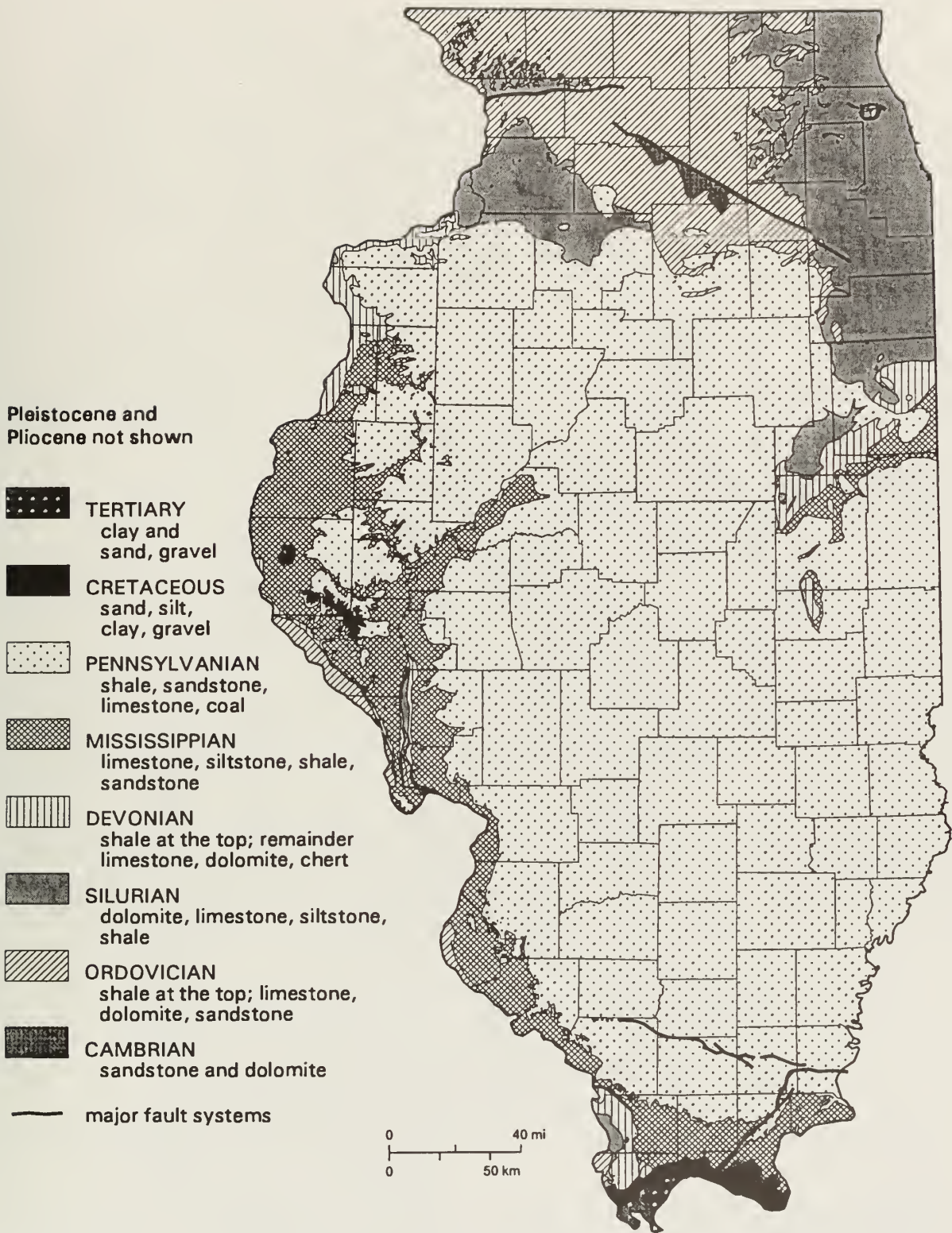
Figure 7 Bedrock geology beneath surficial deposits in Illinois.
