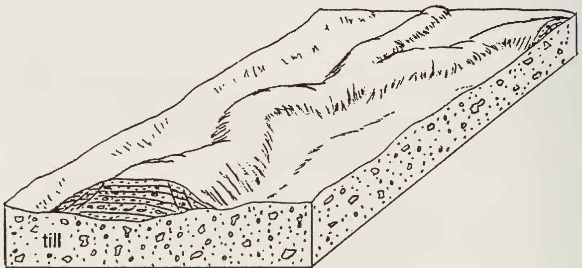
Figure 23 Block diagram of an esker. An esker is formed when a meltwater stream carrying sediment develops beneath a glacier. The stream develops a sinuous pattern as it flows under the ice. When the ice melts, the sediment is left as a long, narrow, winding ridge on the landscape.
