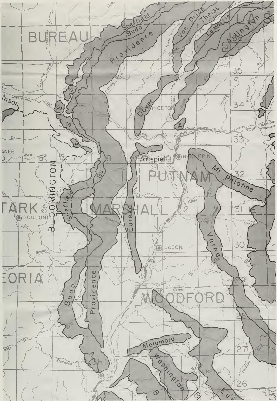
Figure 24 Distribution of Wisconsin Episode moraines in the field trip area (modified from Willman and Frye 1970).
