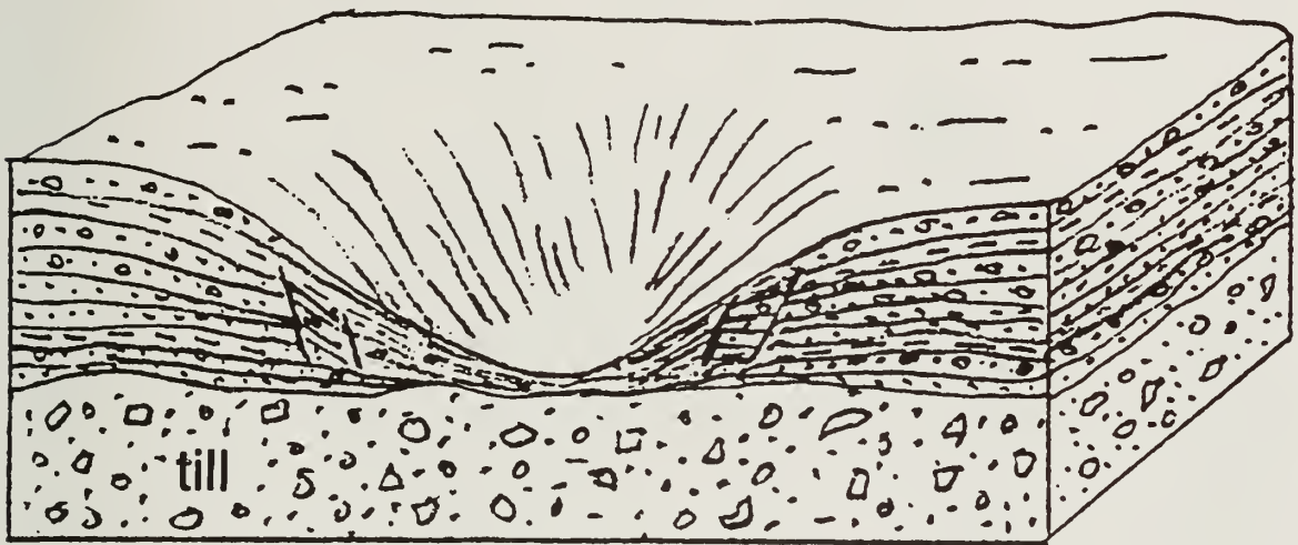
Figure 22 Block diagram of kettle depression. A kettle is formed when a block of ice becomes detached from a glacier and is buried by rock debris deposited by glacial outwash. When the ice block melts, a depression is formed on the landscape.
