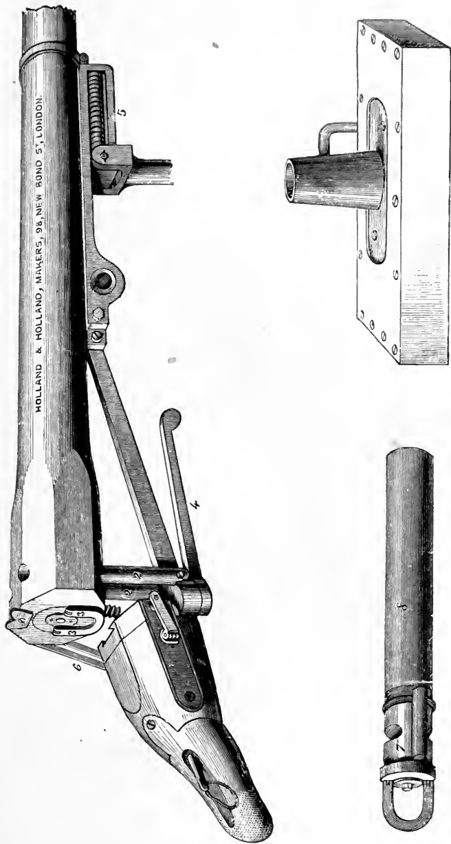
The London Pint Gun, and Mr. E. T. Booth's Recoil Box.
