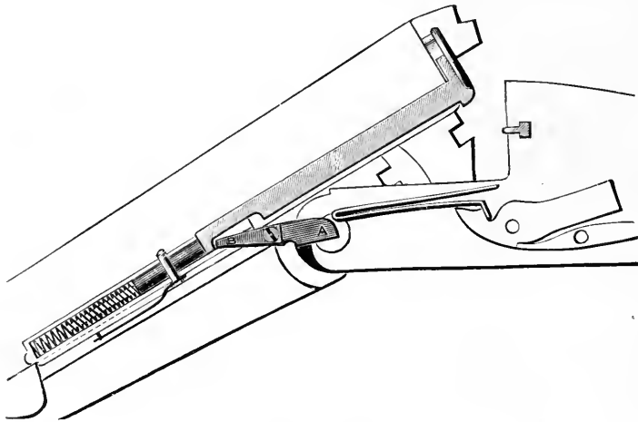
Harrison's Ejector.
