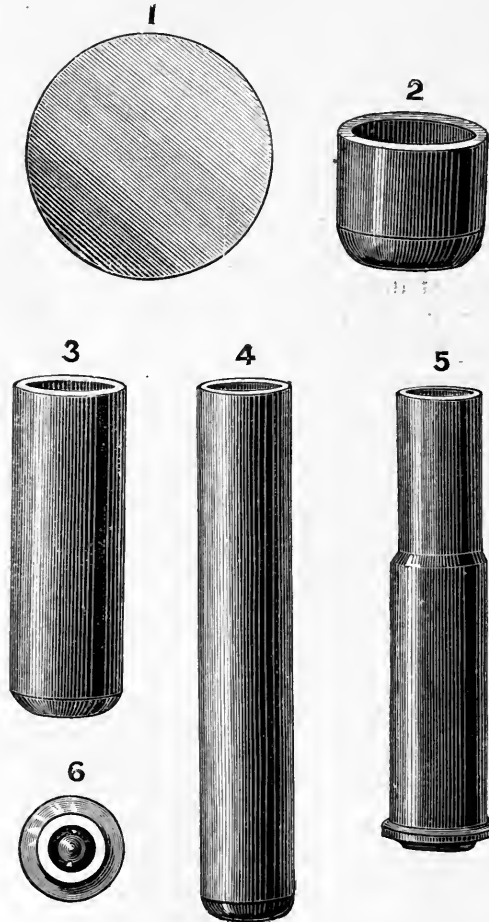
Cartridge Blanks, Cylinder, and Finished Cartridge.
