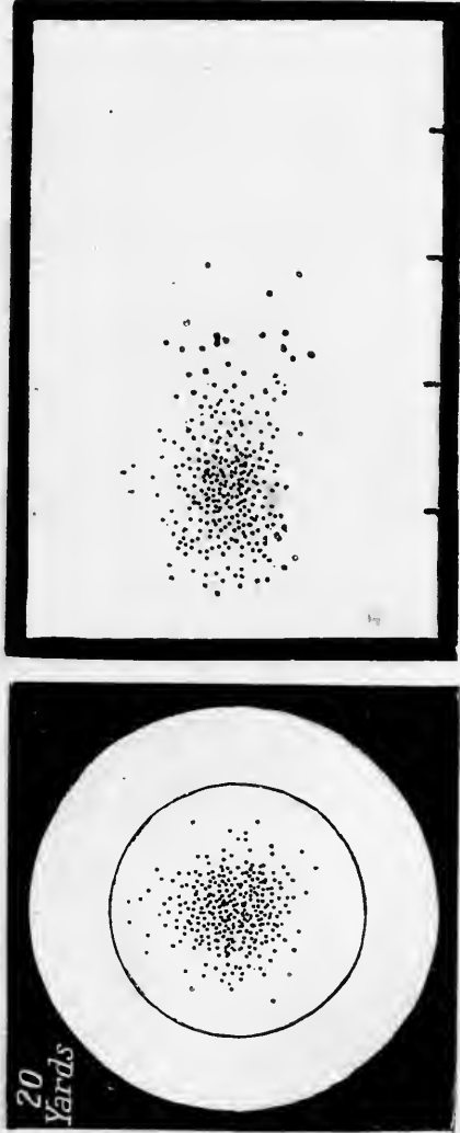
Facsimiles of Patterns showing both Lateral Deviation and Stringing of the same Pellets.
