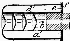
Børrensen's Silencer.
