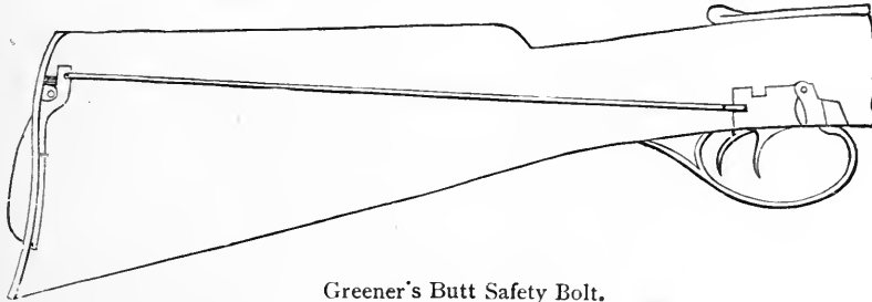
Greener's Butt Safety Bolt.
