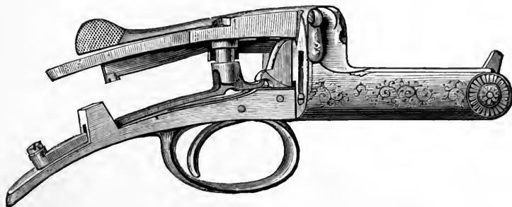
Mechanism of Holland's Hammerless Rook Rifle.
