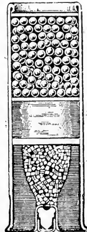
Conical Base, with Balistite Powder.
