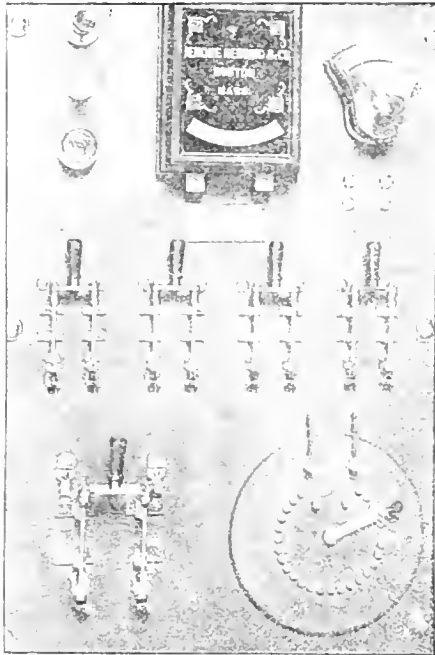
Four Circuit Switch Board for Insulated Electric Light Plant.
