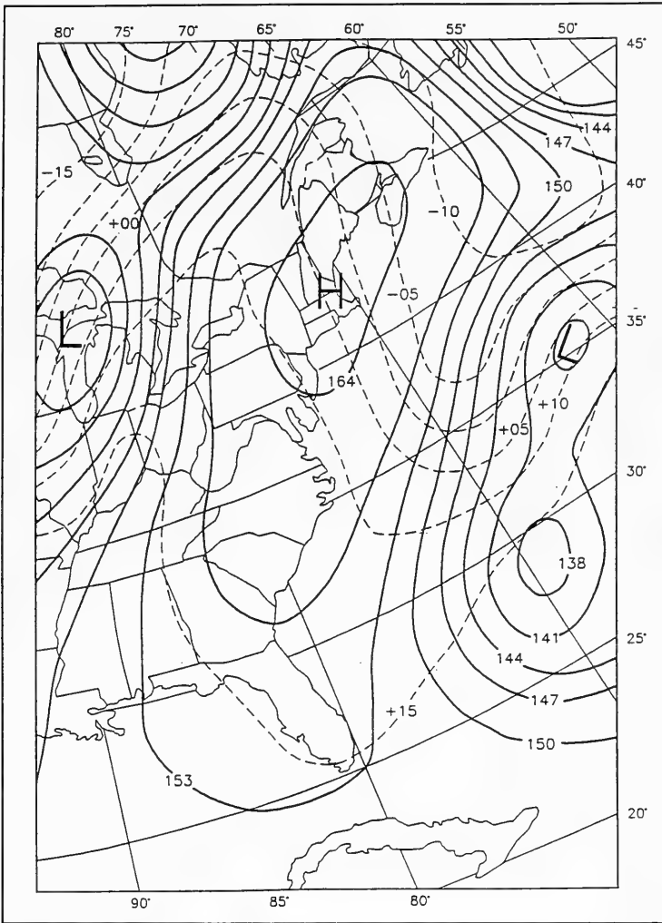
Figure 18. 0000-hr UTC, 29 October 1991, 850-mb height/temperature analysis
