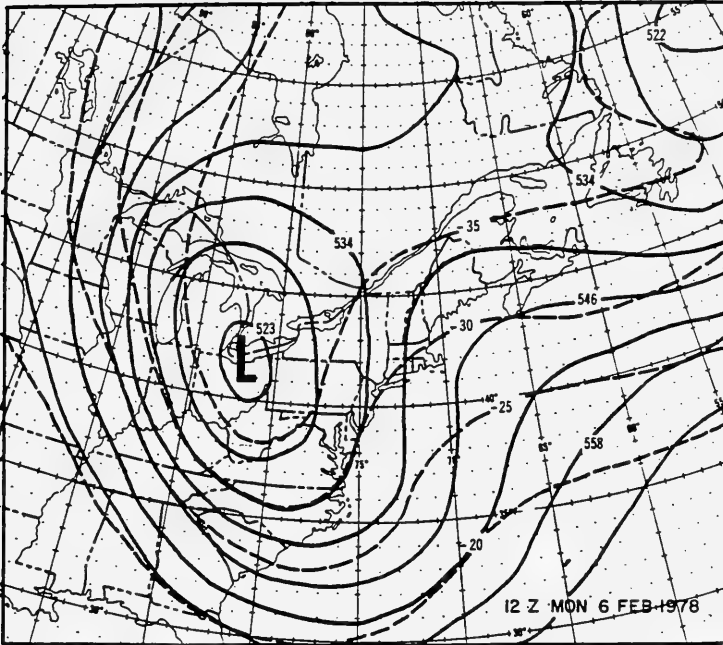
Figure 24. 1200-hr UTC, 6 February 1978, 500-mb height/temperature analysis
