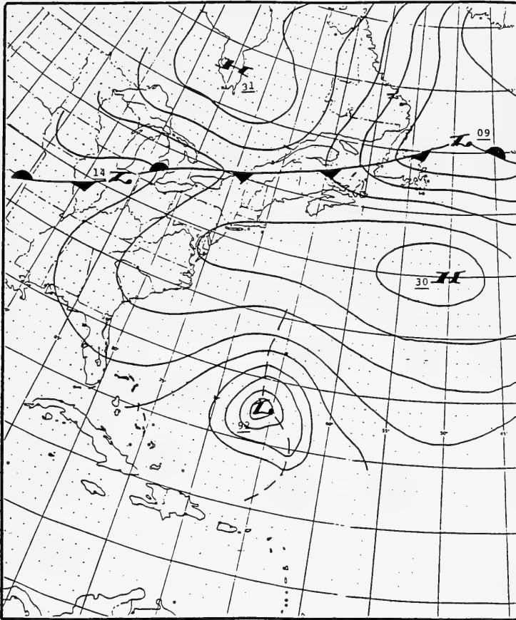
Figure 8. 0000-hr UTC, 27 October 1991, surface analysis
