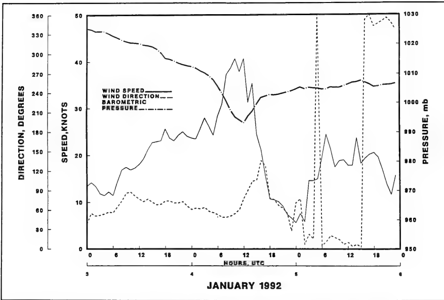
Figure 30. Surface wind data at NDBC buoy 44009 during 4-5 January 1992 storm
