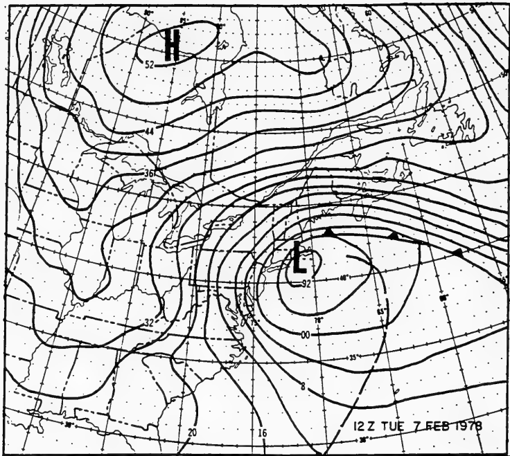
Figure 25. 1200-hr UTC, 7 February 1978, surface analysis
