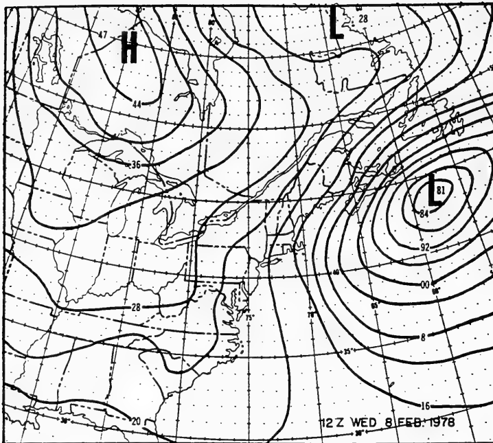
Figure 27. 1200-hr UTC, 8 February 1978, surface analysis
