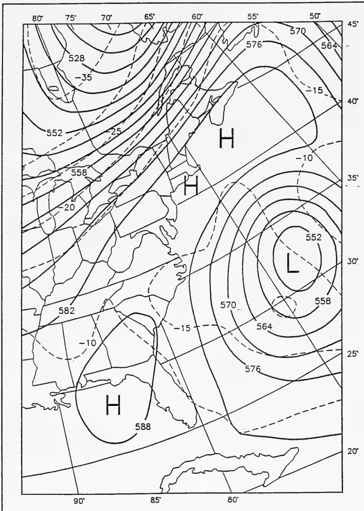
Figure 14. 1200-hr UTC, 30 October 1991, 500-mb height/temperature analysis
