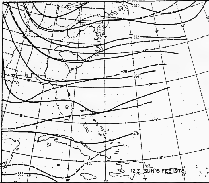
Figure 22. 1200-hr UTC, 5 February 1978, 500-mb height/temperature analysis
