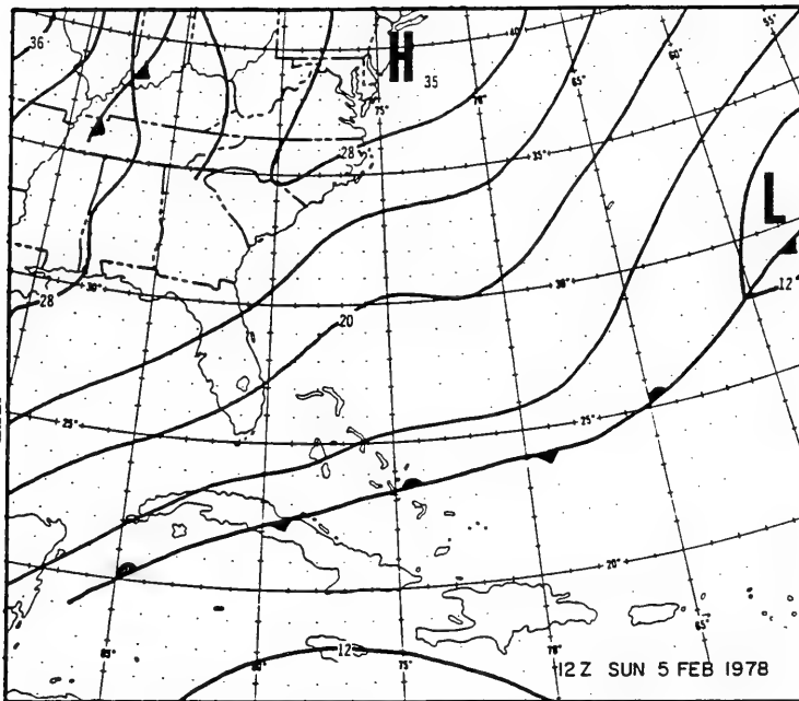
Figure 21. 1200-hr UTC, 5 February 1978, surface analysis
