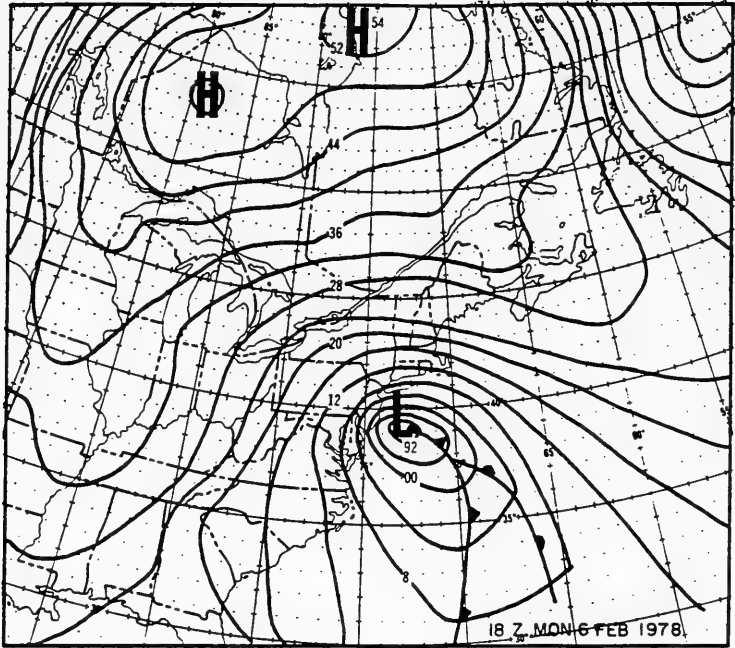
Figure 23. 1800-hr UTC, 6 February 1978, surface analysis
