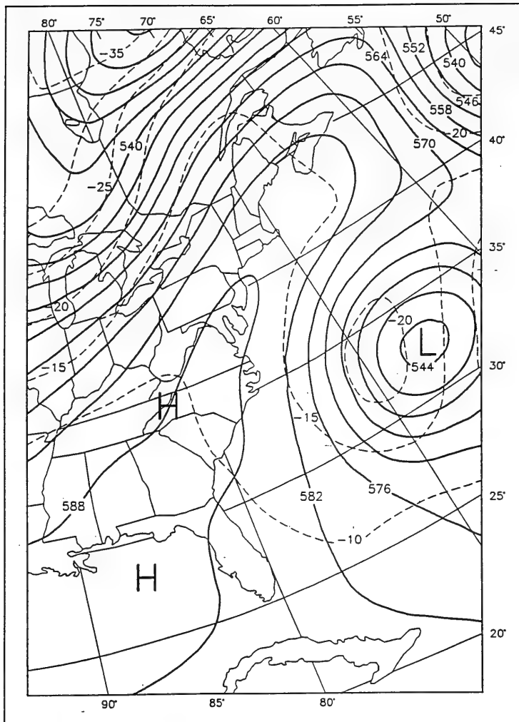
Figure 13. 0000-hr UTC, 30 October 1991, 500-mb height/temperature analysis
