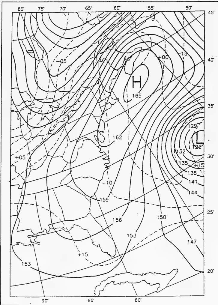
Figure 20. 0000-hr UTC, 30 October 1991, 850-mb height/temperature analysis
