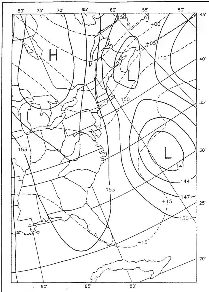
Figure 17. 1200-hr UTC, 28 October 1991, 850-mb height/temperature analysis
