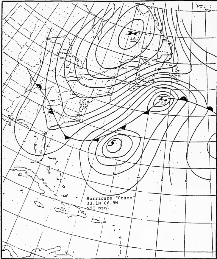
Figure 11. 0000-hr UTC, 29 October 1991, surface analysis
