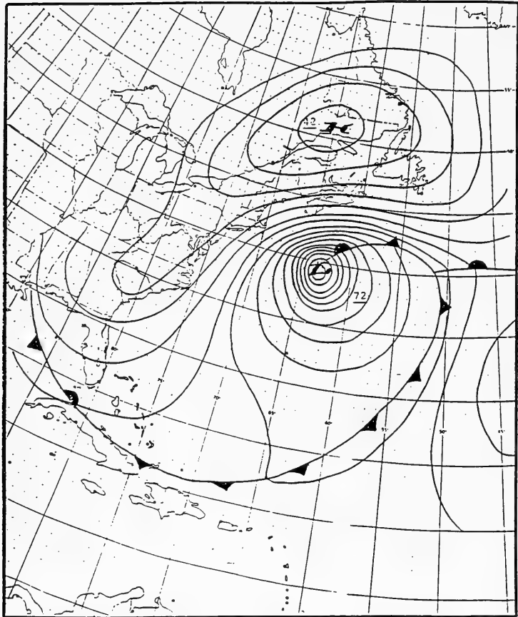
Figure 15. 1200-hr UTC, 30 October 1991, surface analysis
