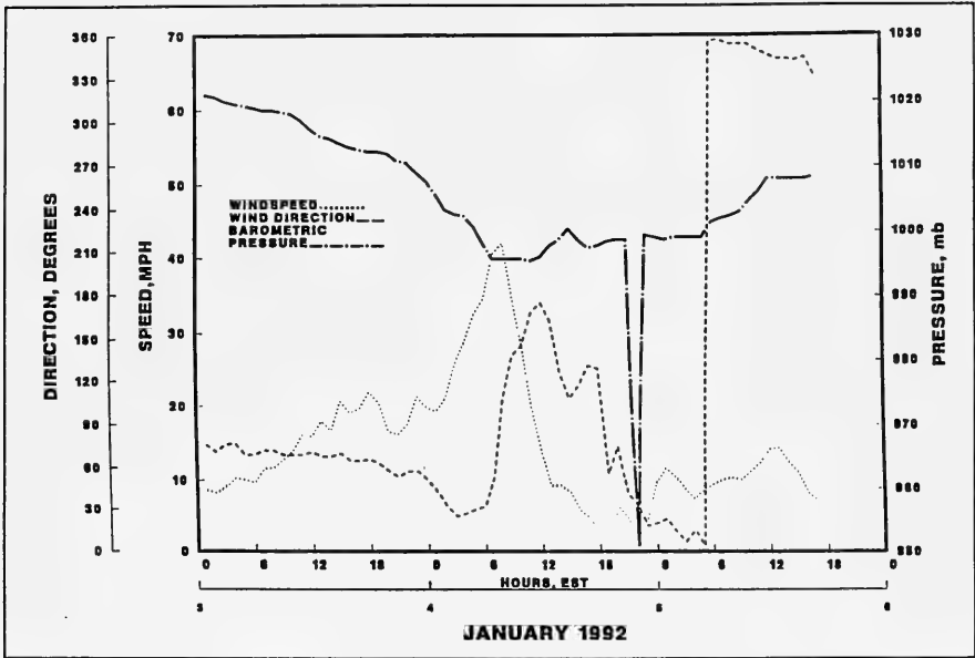
Figure 29. Wind and surface pressure data from National Park Service meteorological station on Assateague Island during 4-5 January 1992 storm
