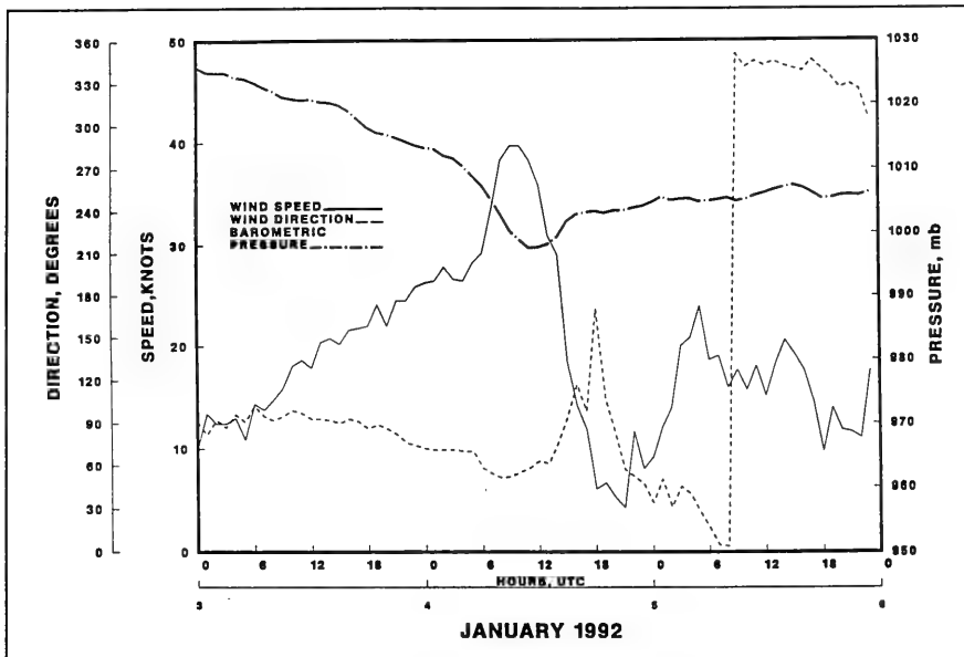
Figure 31. Surface wind data at NDBC buoy 44012 during 4-5 January 1992 storm
