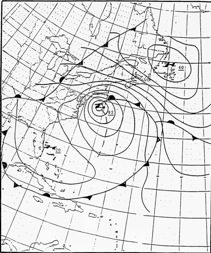
Figure 16. 1200-hr UTC, 31 October 1991, surface analysis
