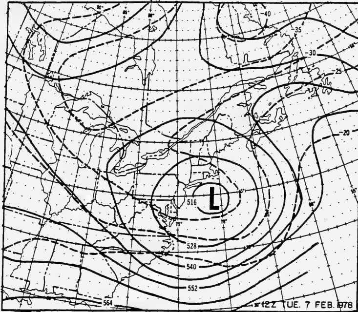
Figure 26. 1200-hr UTC, 7 February 1978, 500-mb height/temperature analysis
