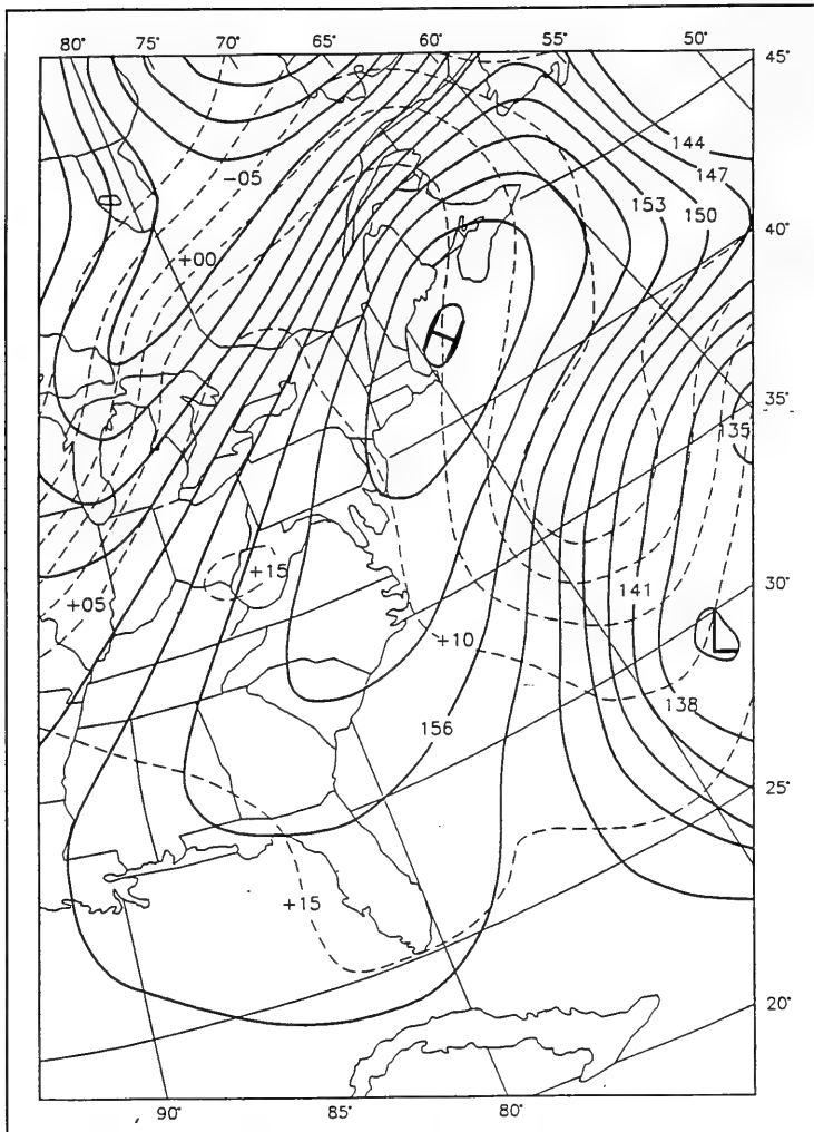
Figure 19. 1200-hr UTC, 29 October 1991, 850-mb height/temperature analysis
