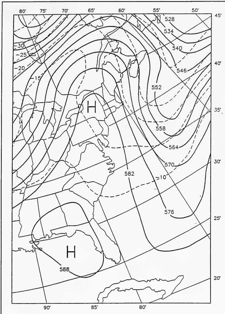
Figure 10. 0000-hr UTC, 29 October 1991, 500-mb height/temperature analysis
