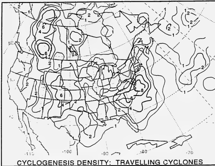
Figure 3. Number of cyclogenesis events per 3 \times 10^5 \text{ km}^2 during GALE, travelling cyclones only (from Neilsen and Dole (1992))
