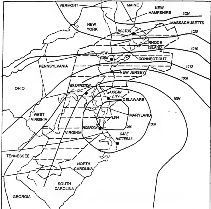
Figure 32. 1220-hr UTC, 4 January 1992, surface pressure analysis
