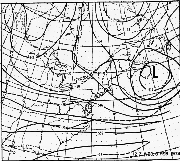
Figure 28. 1200-hr UTC, 8 February 1978, 500-mb height/temperature analysis
