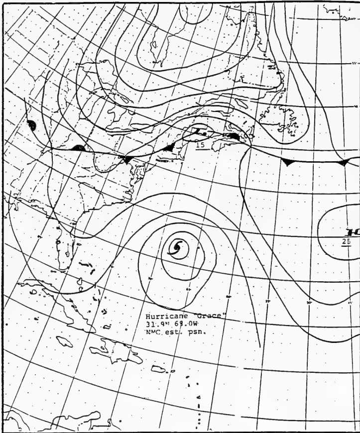
Figure 9. 0000-hr UTC, 28 October 1991, surface analysis
