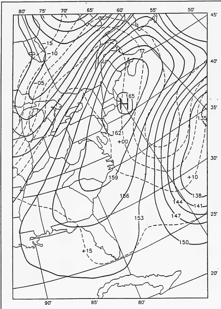
Figure 12. 1200-hr UTC, 29 October 1991, 850-mb height/temperature analysis
