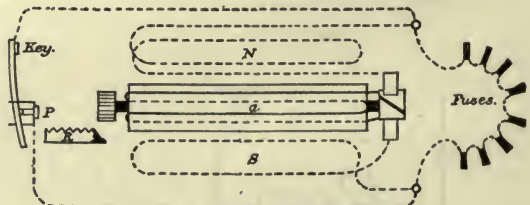
Second View of Circuits.
