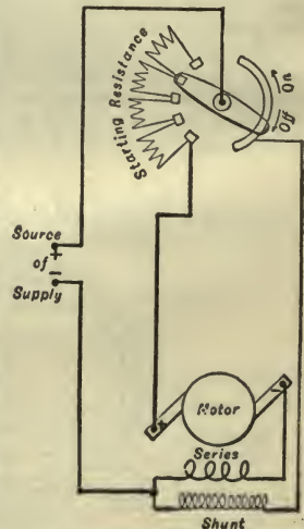
103. Compound Motor.
