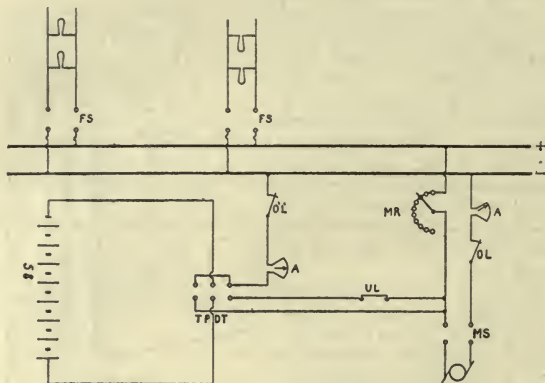
86. Preble Switchboard.
