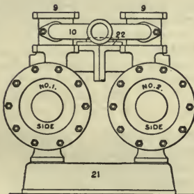
END VIEW OF STEAM CYLINDERS
