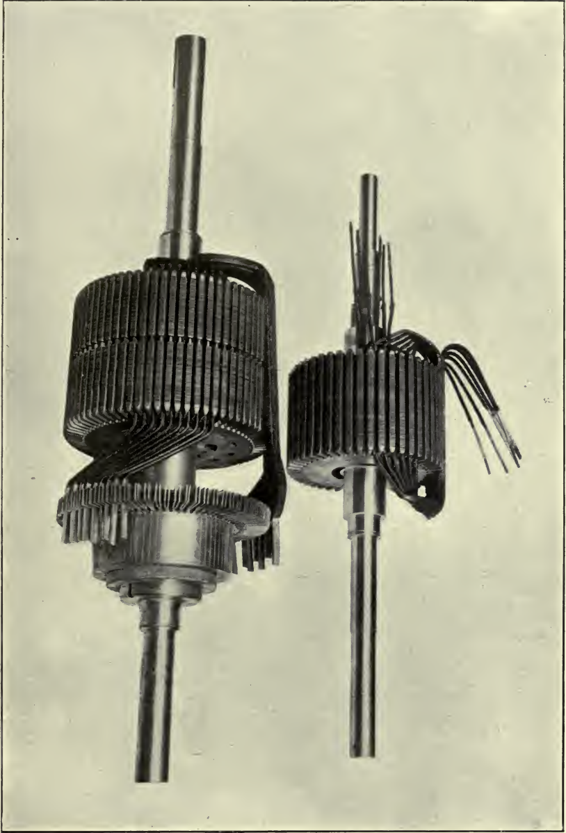
52. W-e Cores, Wave Winding Begun, 4-Pole.
