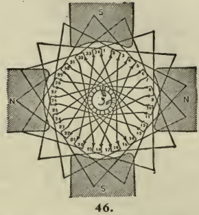
Fig. 46 is a 4-pole, 17-coil, wave, drum winding. Back pitch, 9; front pitch, 9. Two circuits between brushes. Short lines having arrowheads represent wires along the length of the cylinder; outside wires are back connections, inside wires, front connections.
