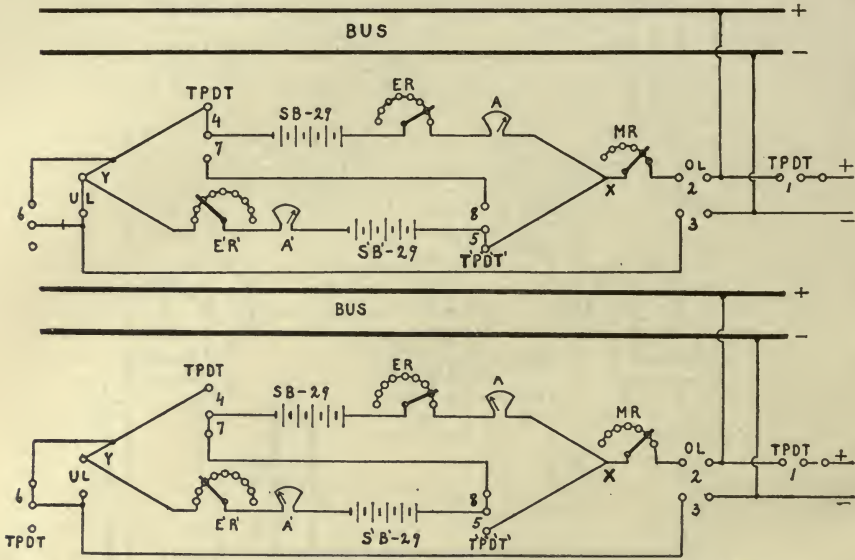
81 and 82. Diagrammatic Sketch of Engineer Switchboard Battery Panel.
