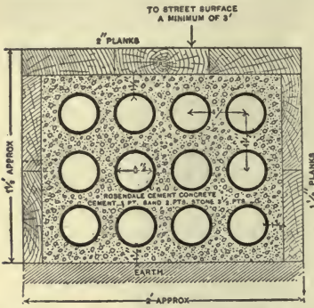
201. Cross-section of Iron-Pipe Conduit.
