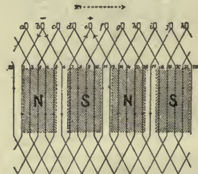
47. Drum Wave Rolled Out.
