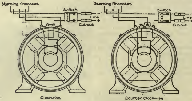
102. Shunt Wound.
