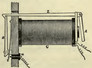
177. Gravity Drop.
