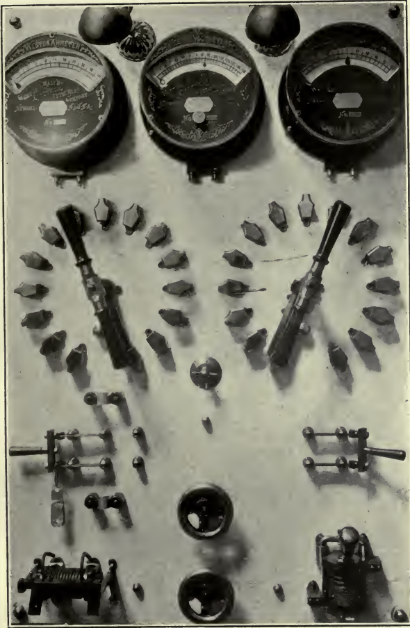
78. W-e Switch Board Front.
