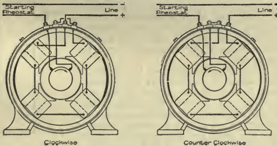
101. Series Wound.
