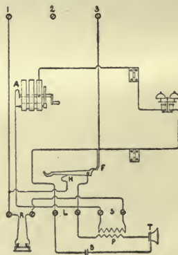
172. Series Telephone Station.
