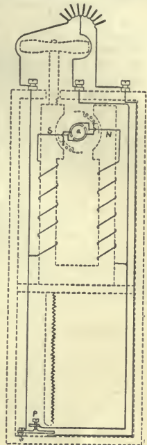
148. 30-Fuse Firing Dynamo.
