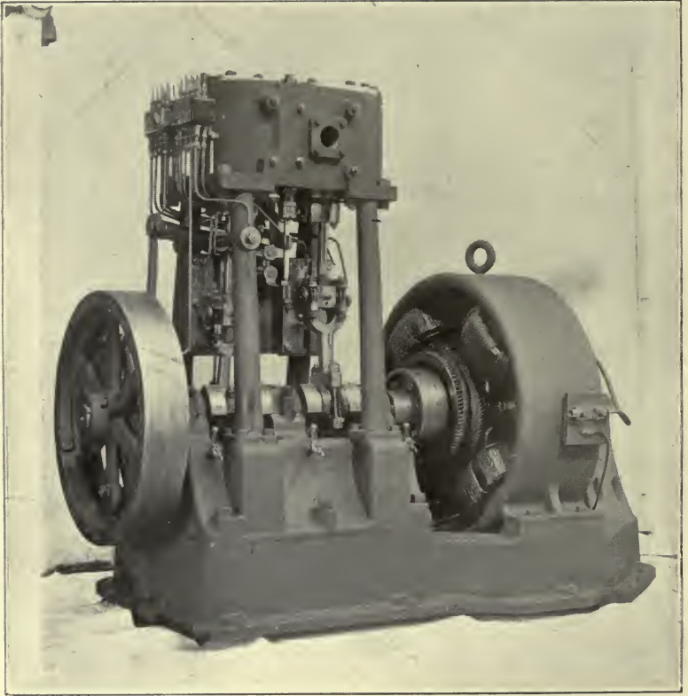
22a. Sturtevant Double Engine.
