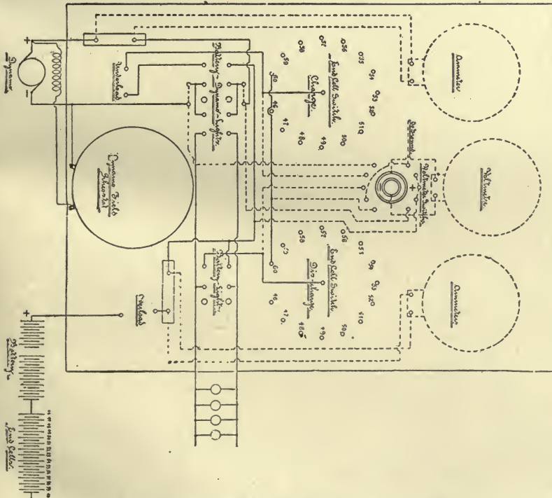
89. Shunt Dynamo, 45 Cells and 15 Active End Cells.
