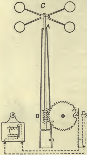
153. Anemometer.
