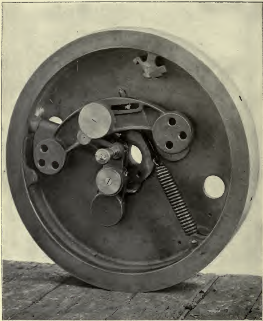
63. Governor.
