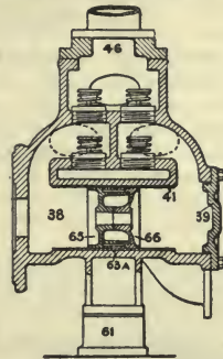
PISTON PATTERN WATER END
