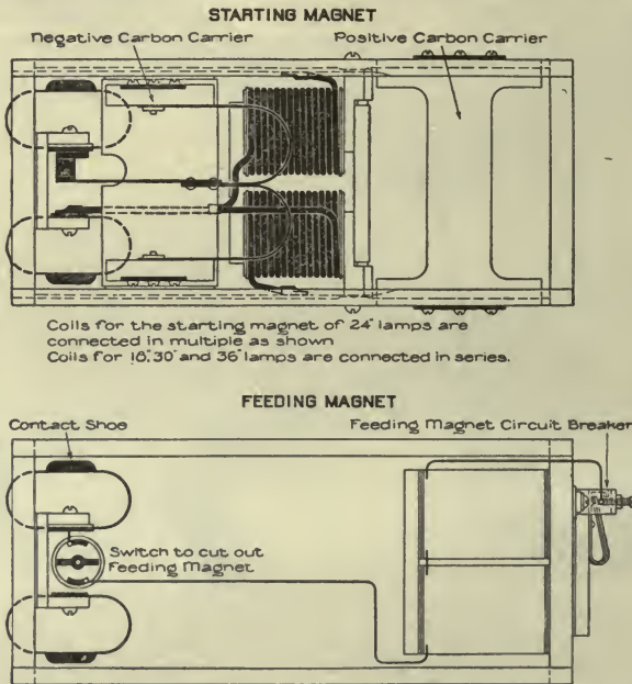
126. Connections of 18, 24, 30 and 36 inch Automatic Projector Lamps.
