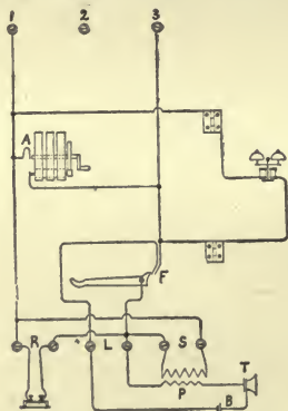
171. Parallel Telephone Station.
