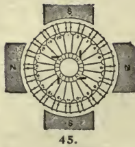
Fig. 45 is a 4-pole, 20-coil, ring, four windings through armature, making its resistance between poles = \frac{1}{16} of that of the single winding. By connecting each bar of the commutator with the one opposite, two brushes 90° apart will be sufficient.
