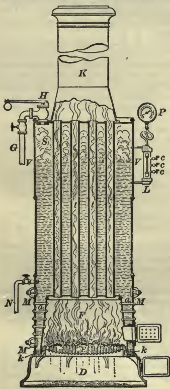
3. Upright Boiler.
