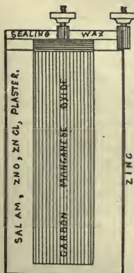
157. Dry Cell.
