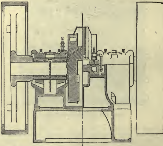
24c. End View Oiling Device.
