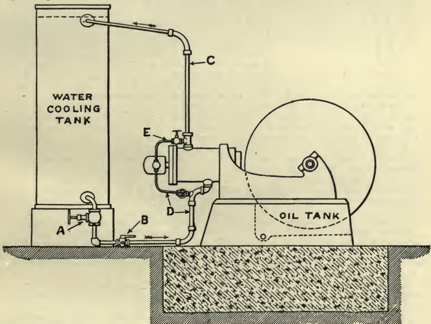
31. Water-Cooling Connections.
