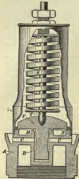
4. Pop Safety Valve.
