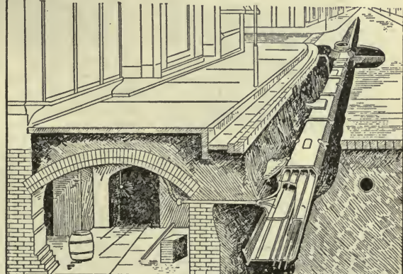
200. Exterior, Wire Conduit in Forts.
