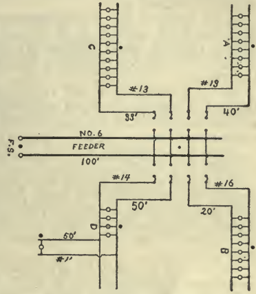
184. How to Find Sizes of Conductors.
