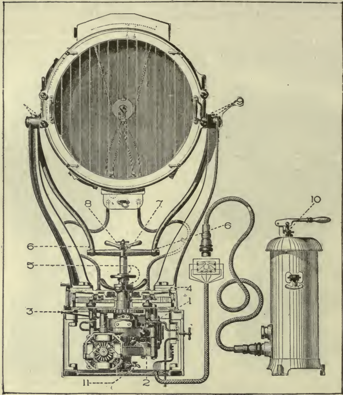
129. Training Mechanism Controller and Cable.
