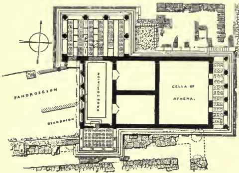
FIG. 115. — The Erechtheum. Plan. (Drawing by G. P. S.)
