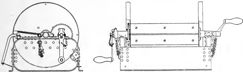
REEL FOR CAISSON, MODEL OF 1917.
