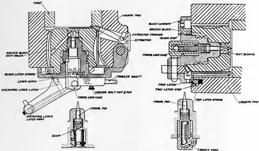
FIRING MECHANISM.
