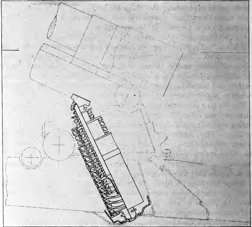
EQUILIBRATOR MECHANISM.
