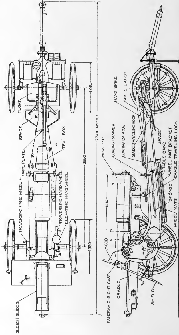
155 MM HOWITZER, MODEL OF 1918 (SCHNEIDER)
