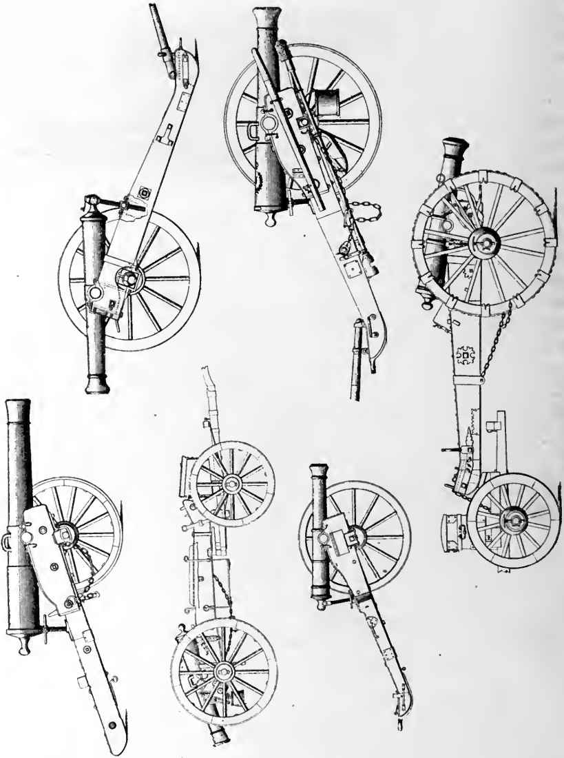
FRENCH ARTILLERY, 1800-1850.
