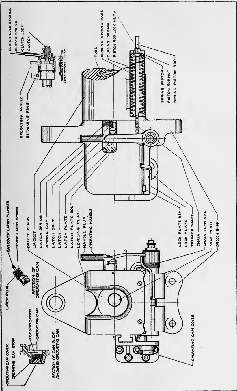
BRECH MECHANISM ASSEMBLY.
