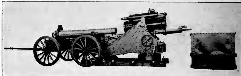
METHOD OF MOUNTING HOWITZER.
