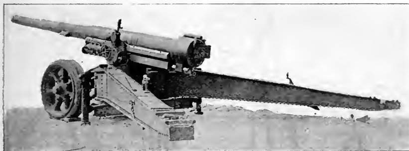
PREPARING CARRIAGE FOR BATTERY POSITION.
