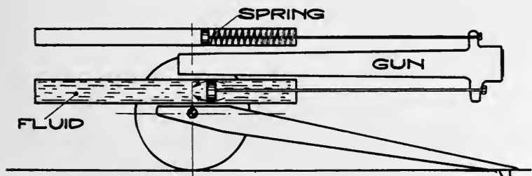
FIG. G END OF RECOIL
