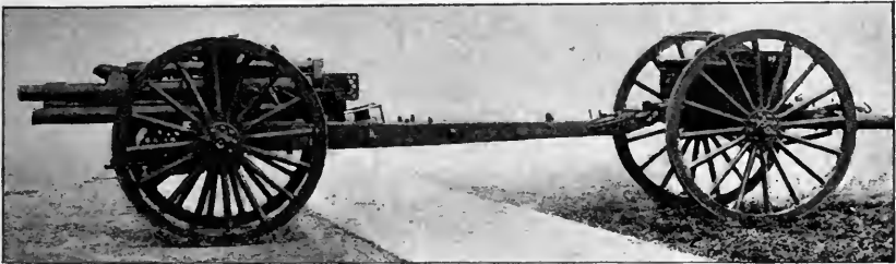
CARRIAGE AND LIMBER IN TRAVELING POSITION.
