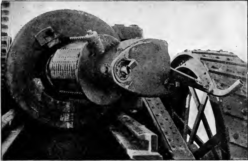
BREECH BLOCK.
