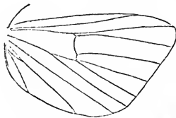
Neuration and head of Eucosma lucunana .
