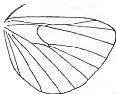
Neuration and head of Pyrausta purpuralis .
