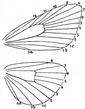
Assumed type of venation of the Lepidoptera .
