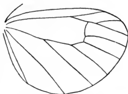
Neuration of Miltochrista senex .
