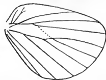
Neuration of Clisiocampa neustria .
