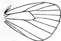
Neuration of Hydriomena pictata .
