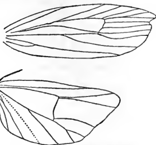
Neuration of Eudemis naevana .
