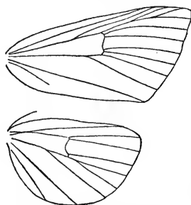
Neuration of Halias prasinana .
