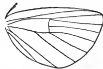
Neuration of Cerura vinula .
