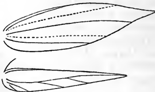
Neuration of Opostega crepusculella .
