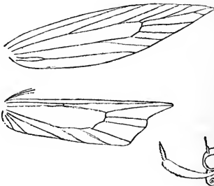
Neuration and head of Parasta neuropterella .
