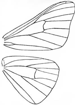
Neuration of Saturnia pavonia .
