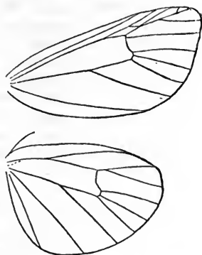
Neuration of Phragmatobia fuliginosa .
