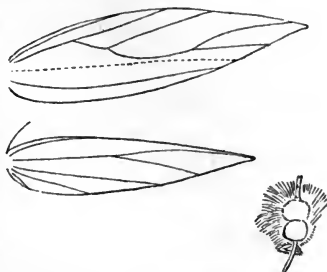
Neuration and head of Nepticula tityrel'a .
