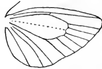
Neuration of Zygaena trifolii .
