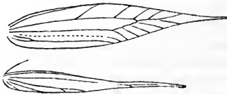
Neuration of Cosmopteryx druryella .
