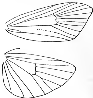
Neuration of Simaethis fabriciana .
