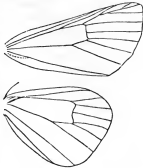
Neuration of Breppos notha .
