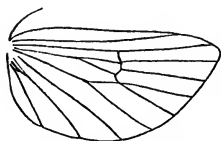
Hindwing of Isotrias hybridana .
