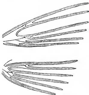
Neuration of Orneodes hexadactyla .
