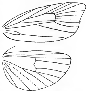
Neuration of Hemimene plumbagana .
