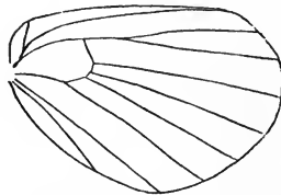
Neuration of Leucophasia sinapis .
