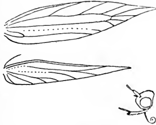
Neuration and head of Coleophora onosmella .
