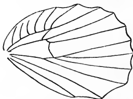
Hindwing of Gastropacha quercifolia .
