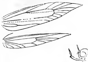
Neuration and head of Epermenia chaerophyllella .
