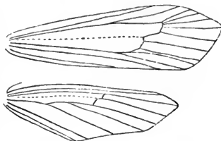
Neuration of Agdistis Bennetii .
