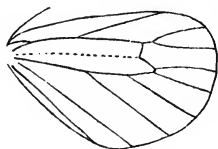
Neuration of Erannis aescularia .
