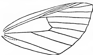
Forewing of Ectropis biundularia .
