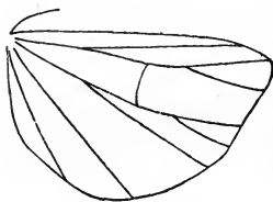
Neuration of Lithosia lurideola : a, portion of ♂ antenna.
