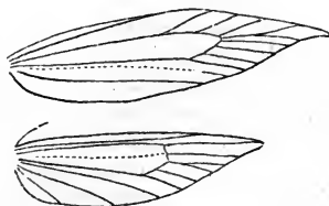
Neuration of Scythrís fuscocuprea .
