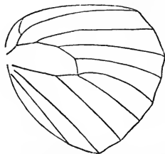
Neuration of Argynnis adippe .
