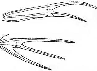
Neuration of Pterophorus spilodactylus .
