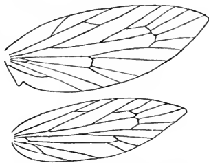
Neuration of Eriocephala calthella .
