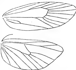
Neuration of Phalonia tesserana .
