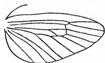
Neuration of Zeuzera pyrina .
