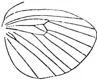
Neuration of Trypanus cossus .
