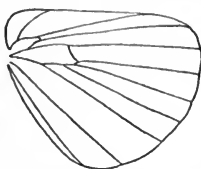
Neuration of Eriogaster rubi .
