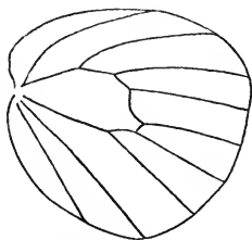
Neuration of Colias edusa .
