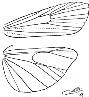
Neuration of Salebria palumbella ; a, base of antenna of ♂.
