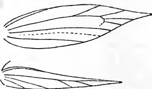
Neuration of Leucoptera laburnella .
