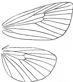
Neuration of Apoda limacodes .
